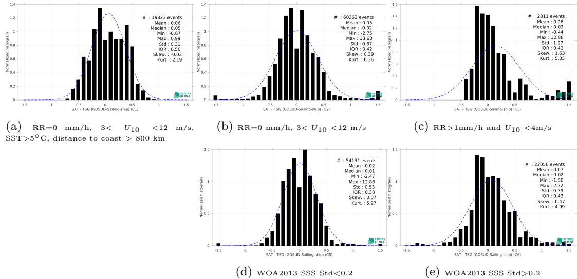
Figure 13: Normalized histogram of \Delta SSS (SMOS SSS L3 v2 - 9-Days (BEC) - TSG (GOSUD-Sailing-ship)) for 5 different subdatasets corresponding to: RR=0 mm/h, 3 < U_{10} < 12 m/s, SST >5^\circ C, distance to coast > 800 km (a), RR=0 mm/h, 3 < U_{10} < 12 m/s (b), RR >1 mm/h and U_{10} < 4 m/s (c), WOA2013 SSS Std <0.2 (d), WOA2013 SSS Std >0.2 (e).
