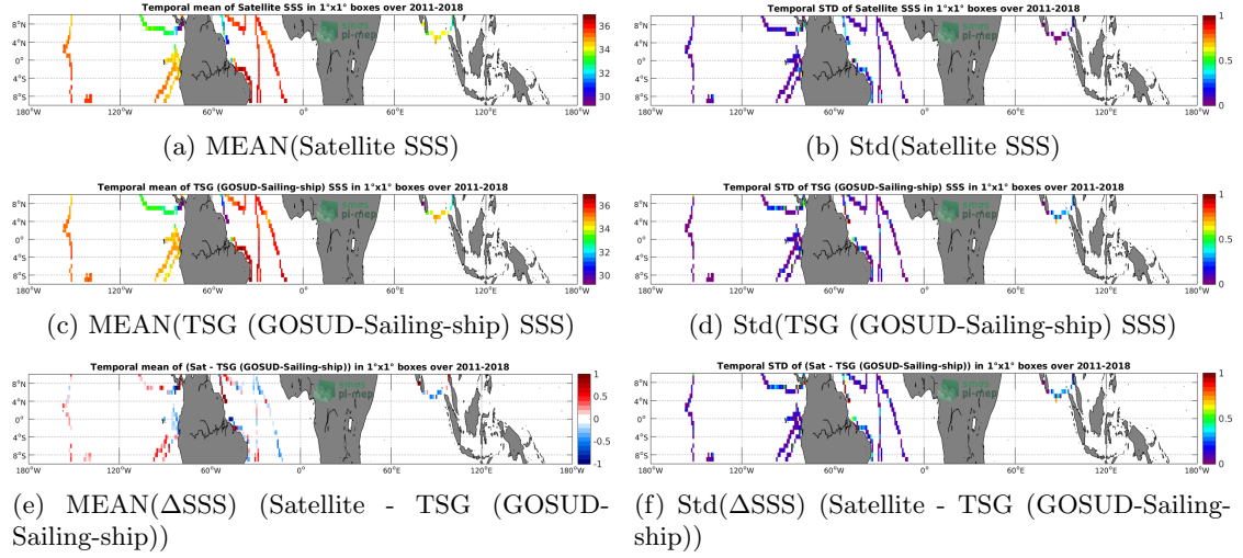
Figure 6: Temporal mean (left) and Std (right) of SSS from SMOS SSS L3 v2 - 9-Days (BEC) (top), TSG (GOSUD-Sailing-ship) (middle), and of \Delta SSS (Satellite - TSG (GOSUD-Sailing-ship)). Only match-up pairs are used to generate these maps.
