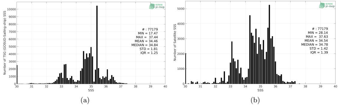
Figure 2: Histograms of SSS from TSG (GOSUD-Sailing-ship) (a) and SMOS SSS L3 v2 - 9-Days (BEC) (b) considering all match-up pairs per bins of 0.1 over the Equatorial Ocean 10N-10S Pi-MEP region and for the full satellite product period.
