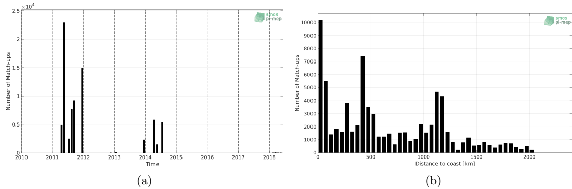
Figure 1: Number of match-ups between TSG (GOSUD-Sailing-ship) and SMOS SSS L3 v2 - 9-Days (BEC) SSS as a function of time (a) and as function of the distance to coast (b) over the Equatorial Ocean 10N-10S Pi-MEP region and for the full satellite product period.
