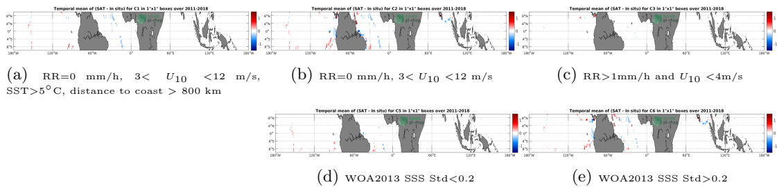
Figure 12: Temporal mean gridded over spatial boxes of size 1^\circ \times 1^\circ of \Delta SSS (SMOS SSS L3 v2 - 9-Days (BEC) - TSG (GOSUD-Sailing-ship)) for 5 different subdatasets corresponding to: RR=0 mm/h, 3 < U_{10} < 12 m/s, SST>5°C, distance to coast > 800 km (a), RR=0 mm/h, 3 < U_{10} < 12 m/s (b), RR>1mm/h and U_{10} < 4 m/s (c), WOA2013 SSS Std<0.2 (d), WOA2013 SSS Std>0.2 (e).
