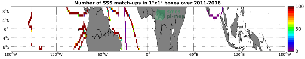
Figure 4: Number of SSS match-ups between TSG (GOSUD-Sailing-ship) SSS and the SMOS SSS L3 v2 - 9-Days (BEC) SSS product for the Equatorial Ocean 10N-10S Pi-MEP region over 1^\circ \times 1^\circ boxes and for the full satellite product period.
