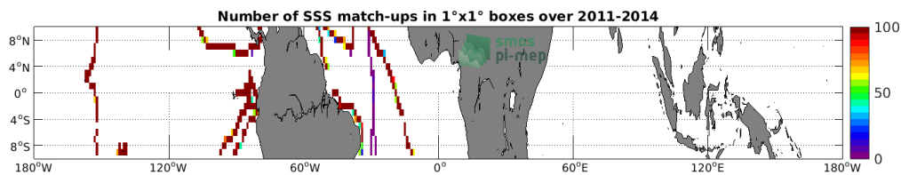
Figure 4: Number of SSS match-ups between TSG (GOSUD-Sailing-ship) SSS and the SMOS SSS L3 v2 - 9-Days (BEC) SSS product for the Equatorial Ocean 10N-10S Pi-MEP region over 1°x1° boxes and for the full satellite product period.
