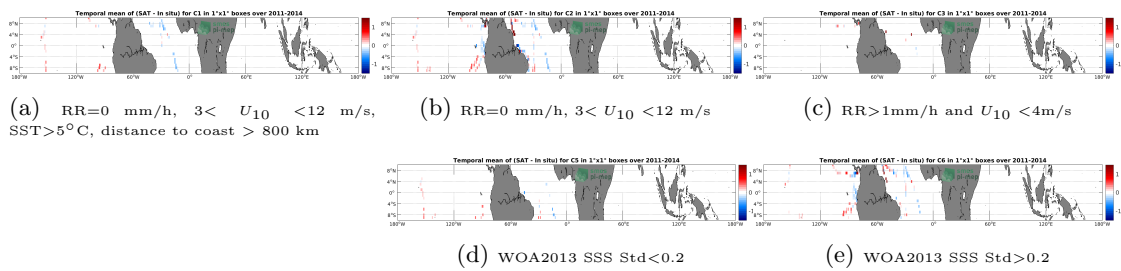
Figure 12: Temporal mean gridded over spatial boxes of size 1°x1° of ΔSSS (SMOS SSS L3 v2 - 9-Days (BEC) - TSG (GOSUD-Sailing-ship)) for 5 different subdatasets corresponding to:RR=0 mm/h, 3 < U_{10} < 12 m/s, SST>5°C, distance to coast > 800 km (a), RR=0 mm/h, 3 < U_{10} < 12 m/s (b), RR>1mm/h and U_{10} < 4 m/s (c), WOA2013 SSS Std<0.2 (d), WOA2013 SSS Std>0.2 (e).
