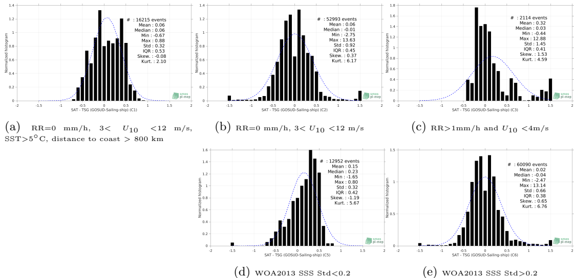
Figure 13: Normalized histogram of ΔSSS (SMOS SSS L3 v2 - 9-Days (BEC) - TSG (GOSUD-Sailing-ship)) for 5 different subdatasets corresponding to: RR=0 mm/h, 3 < U_{10} < 12 m/s, SST>5°C, distance to coast > 800 km (a), RR=0 mm/h, 3 < U_{10} < 12 m/s (b), RR>1mm/h and U_{10} < 4 m/s (c), WOA2013 SSS Std<0.2 (d), WOA2013 SSS Std>0.2 (e).
