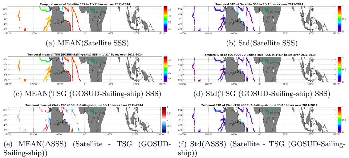
Figure 6: Temporal mean (left) and Std (right) of SSS from SMOS L3 v2 - 9-Days (BEC) (top), TSG (GOSUD-Sailing-ship) (middle), and of \Delta SSS (Satellite - TSG (GOSUD-Sailing-ship)). Only match-up pairs are used to generate these maps.
