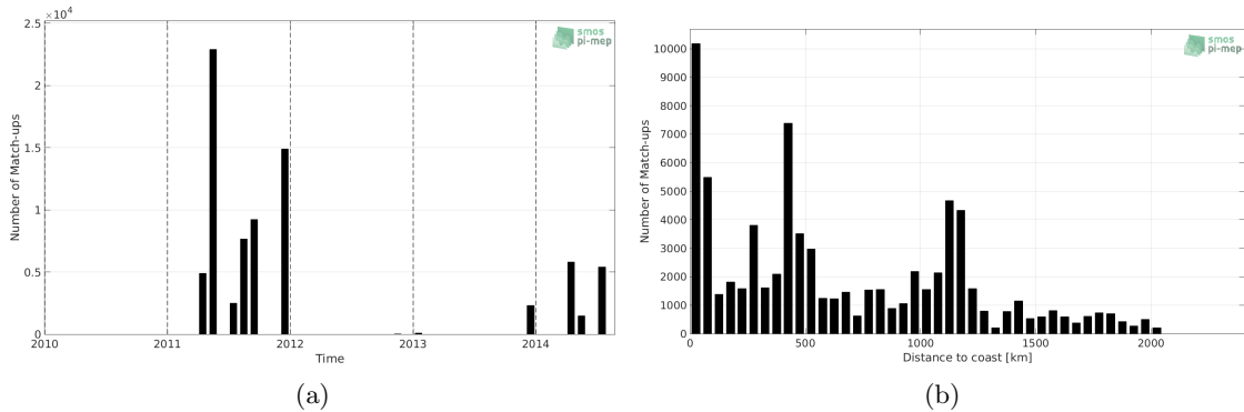
Figure 1: Number of match-ups between TSG (GOSUD-Sailing-ship) and SMOS L3 v2 - 9-Days (BEC) SSS as a function of time (a) and as function of the distance to coast (b) over the Equatorial Ocean 10N-10S Pi-MEP region and for the full satellite product period.
