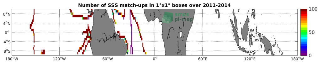
Figure 4: Number of SSS match-ups between TSG (GOSUD-Sailing-ship) SSS and the SMOS L3 v2 - 9-Days (BEC) SSS product for the Equatorial Ocean 10N-10S Pi-MEP region over 1°x1° boxes and for the full satellite product period.
