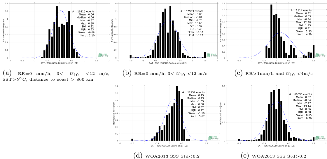
Figure 13: Normalized histogram of ΔSSS (SMOS L3 v2 - 9-Days (BEC) - TSG (GOSUD-Sailing-ship)) for 5 different subdatasets corresponding to: RR=0 mm/h, 3 < U 10 < 12 m/s, SST>5°C, distance to coast > 800 km (a), RR=0 mm/h, 3 < U 10 < 12 m/s (b), RR>1mm/h and U 10 < 4m/s (c), WOA2013 SSS Std<0.2 (d), WOA2013 SSS Std>0.2 (e).
