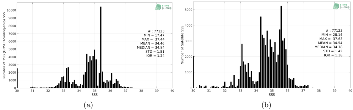
Figure 2: Histograms of SSS from TSG (GOSUD-Sailing-ship) (a) and SMOS L3 v2 - 9-Days (BEC) (b) considering all match-up pairs per bins of 0.1 over the Equatorial Ocean 10N-10S Pi-MEP region and for the full satellite product period.
