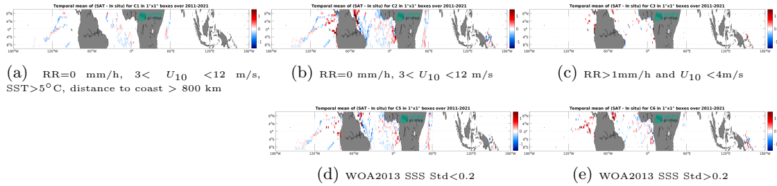
Figure 14: Temporal mean gridded over spatial boxes of size 1^\circ \times 1^\circ of \Delta SSS (SMOS SSS L3 v2 - 9-Days (BEC) - TSG (GOSUD-Research-vessel)) for 5 different subdatasets corresponding to: RR=0 mm/h, 3 < U_{10} < 12 m/s, SST >5^\circ\text{C} , distance to coast > 800 km (a), RR=0 mm/h, 3 < U_{10} < 12 m/s (b), RR >1 mm/h and U_{10} < 4 m/s (c), WOA2013 SSS Std <0.2 (d), WOA2013 SSS Std >0.2 (e).
