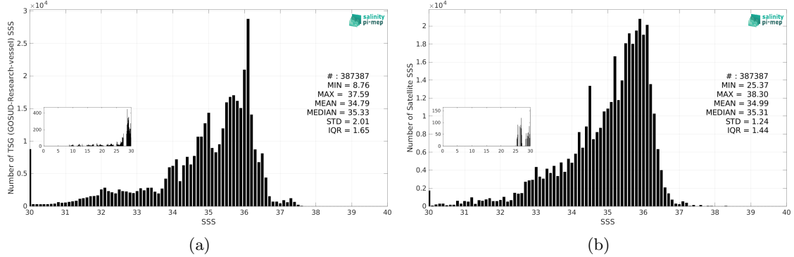
Figure 3: Histograms of SSS from TSG (GOSUD-Research-vessel) (a) and SMOS SSS L3 v2 - 9-Days (BEC) (b) considering all match-up pairs per bins of 0.1 over the Equatorial Ocean 10N-10S Pi-MEP region and for the full satellite product period.
