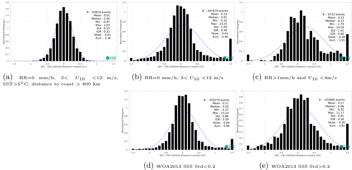
Figure 15: Normalized histogram of \Delta SSS (SMOS SSS L3 v2 - 9-Days (BEC) - TSG (GOSUD-Research-vessel)) for 5 different subdatasets corresponding to: RR=0 mm/h, 3 < U_{10} < 12 m/s, SST >5^\circ\text{C} , distance to coast > 800 km (a), RR=0 mm/h, 3 < U_{10} < 12 m/s (b), RR >1 mm/h and U_{10} < 4 m/s (c), WOA2013 SSS Std <0.2 (d), WOA2013 SSS Std >0.2 (e).
