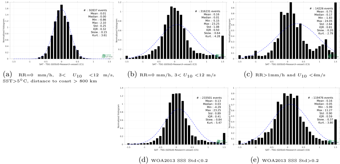
Figure 13: Normalized histogram of \Delta SSS (SMOS SSS L3 v2 - 9-Days (BEC) - TSG (GOSUD-Research-vessel)) for 5 different subdatasets corresponding to: RR=0 mm/h, 3 < U_{10} < 12 m/s, SST >5^\circ C, distance to coast > 800 km (a), RR=0 mm/h, 3 < U_{10} < 12 m/s (b), RR >1 mm/h and U_{10} < 4 m/s (c), WOA2013 SSS Std <0.2 (d), WOA2013 SSS Std >0.2 (e).
