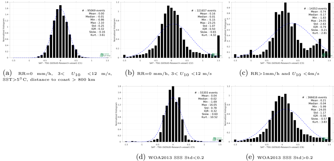
Figure 13: Normalized histogram of \Delta\text{SSS} (SMOS SSS L3 v2 - 9-Days (BEC) - TSG (GOSUD-Research-vessel)) for 5 different subdatasets corresponding to: RR=0 mm/h, 3 < U_{10} < 12 m/s, SST>5°C, distance to coast > 800 km (a), RR=0 mm/h, 3 < U_{10} < 12 m/s (b), RR>1mm/h and U_{10} < 4 m/s (c), WOA2013 SSS Std<0.2 (d), WOA2013 SSS Std>0.2 (e).
