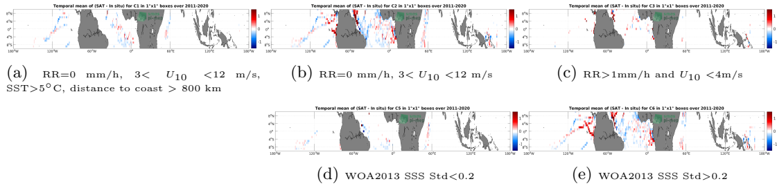
Figure 12: Temporal mean gridded over spatial boxes of size 1^\circ \times 1^\circ of \Delta\text{SSS} (SMOS SSS L3 v2 - 9-Days (BEC) - TSG (GOSUD-Research-vessel)) for 5 different subdatasets corresponding to: RR=0 mm/h, 3 < U_{10} < 12 m/s, SST>5°C, distance to coast > 800 km (a), RR=0 mm/h, 3 < U_{10} < 12 m/s (b), RR>1mm/h and U_{10} < 4 m/s (c), WOA2013 SSS Std<0.2 (d), WOA2013 SSS Std>0.2 (e).
