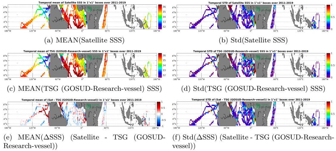
Figure 6: Temporal mean (left) and Std (right) of SSS from SMOS SSS L3 v2 - 9-Days (BEC) (top), TSG (GOSUD-Research-vessel) (middle), and of \Delta SSS (Satellite - TSG (GOSUD-Research-vessel)). Only match-up pairs are used to generate these maps.
