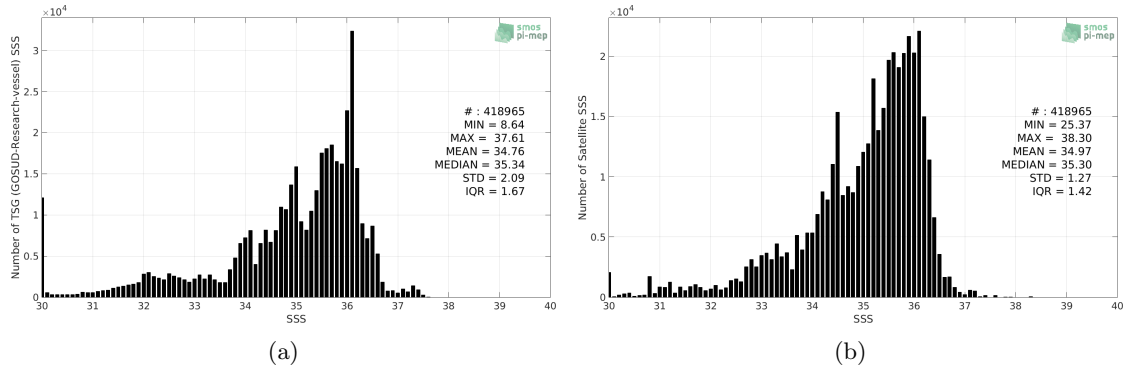
Figure 2: Histograms of SSS from TSG (GOSUD-Research-vessel) (a) and SMOS SSS L3 v2 - 9-Days (BEC) (b) considering all match-up pairs per bins of 0.1 over the Equatorial Ocean 10N-10S Pi-MEP region and for the full satellite product period.
