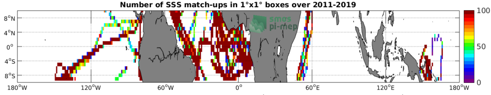
Figure 4: Number of SSS match-ups between TSG (GOSUD-Research-vessel) SSS and the SMOS SSS L3 v2 - 9-Days (BEC) SSS product for the Equatorial Ocean 10N-10S Pi-MEP region over 1^\circ \times 1^\circ boxes and for the full satellite product period.
