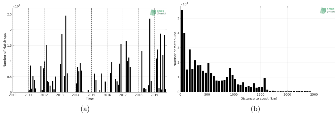
Figure 1: Number of match-ups between TSG (GOSUD-Research-vessel) and SMOS SSS L3 v2 - 9-Days (BEC) SSS as a function of time (a) and as function of the distance to coast (b) over the Equatorial Ocean 10N-10S Pi-MEP region and for the full satellite product period.
