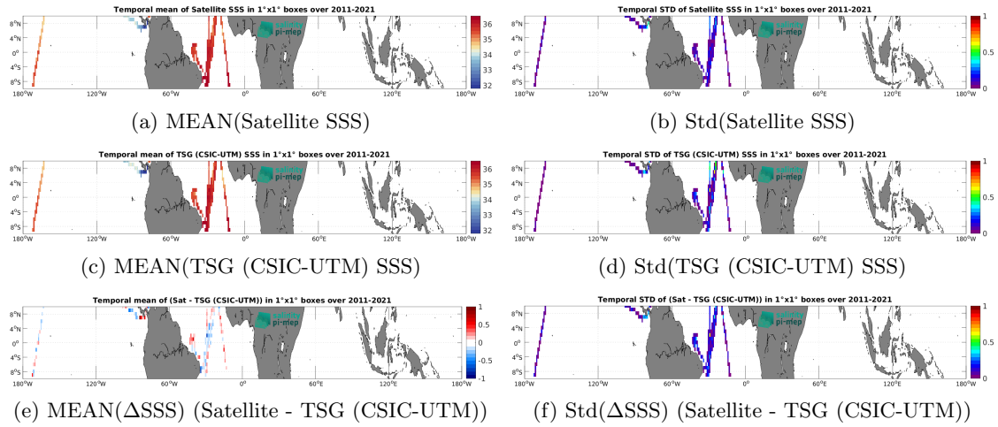
Figure 7: Temporal mean (left) and Std (right) of SSS from SMOS SSS L3 v2 - 9-Days (BEC) (top), TSG (CSIC-UTM) (middle), and of \Delta SSS (Satellite - TSG (CSIC-UTM)). Only match-up pairs are used to generate these maps.
