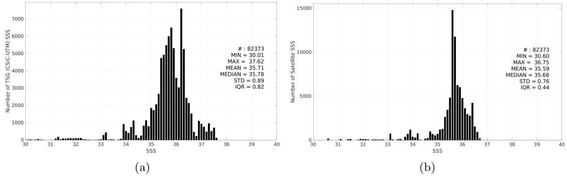
Figure 3: Histograms of SSS from TSG (CSIC-UTM) (a) and SMOS SSS L3 v2 - 9-Days (BEC) (b) considering all match-up pairs per bins of 0.1 over the Equatorial Ocean 10N-10S Pi-MEP region and for the full satellite product period.
