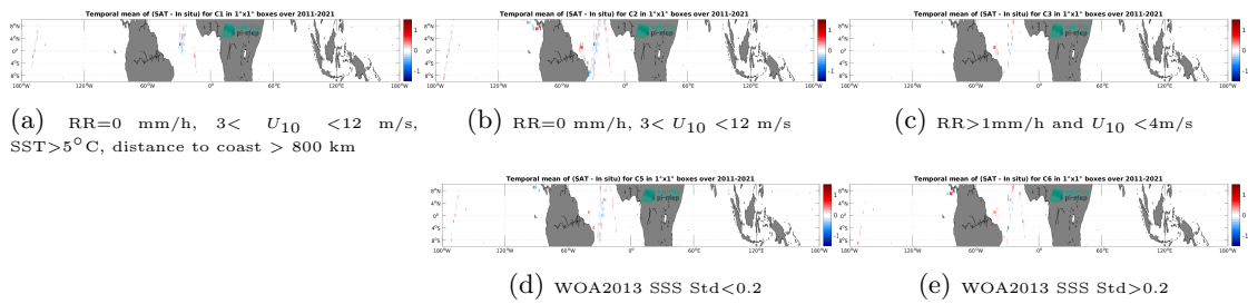
Figure 14: Temporal mean gridded over spatial boxes of size 1^\circ \times 1^\circ of \Delta SSS (SMOS SSS L3 v2 - 9-Days (BEC) - TSG (CSIC-UTM)) for 5 different subdatasets corresponding to:RR=0 mm/h, 3 < U_{10} < 12 m/s, SST>5°C, distance to coast > 800 km (a), RR=0 mm/h, 3 < U_{10} < 12 m/s (b), RR>1mm/h and U_{10} < 4 m/s (c), WOA2013 SSS Std<0.2 (d), WOA2013 SSS Std>0.2 (e).
