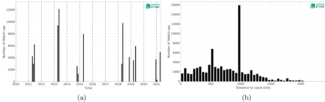
Figure 2: Number of match-ups between TSG (CSIC-UTM) and SMOS SSS L3 v2 - 9-Days (BEC) SSS as a function of time (a) and as function of the distance to coast (b) over the Equatorial Ocean 10N-10S Pi-MEP region and for the full satellite product period.
