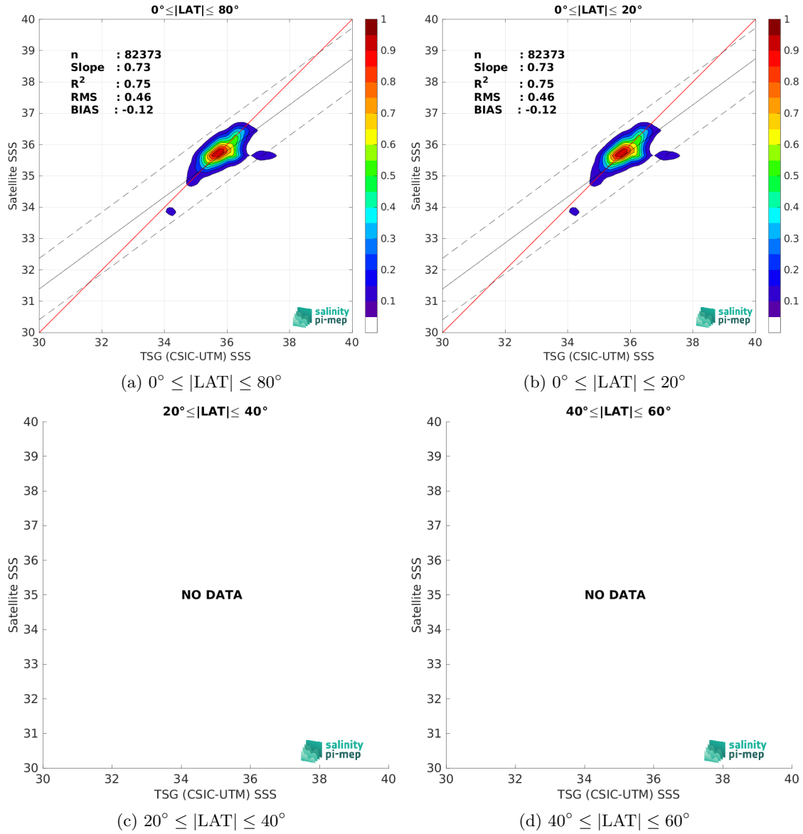
Figure 10: Contour maps of the concentration of SMOS SSS L3 v2 - 9-Days (BEC) SSS (y-axis) versus TSG (CSIC-UTM) SSS (x-axis) at match-up pairs for different latitude bands. For each plot, the red line shows x=y . The black thin and dashed lines indicate a linear fit through the data cloud and the \pm 95\% confidence levels, respectively. The number match-up pairs n , the slope and R^2 coefficient of the linear fit, the root mean square (RMS) and the mean bias between satellite and in situ data are indicated for each latitude band in each plots.
