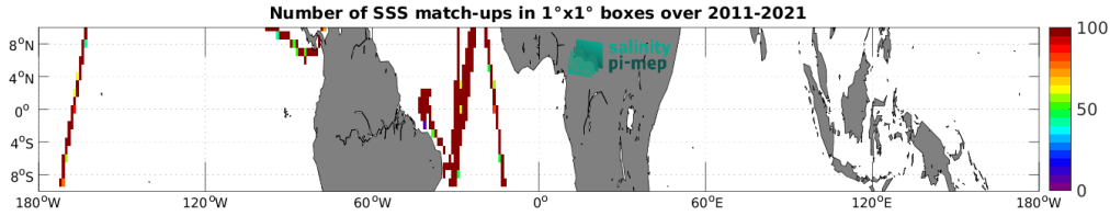
Figure 5: Number of SSS match-ups between TSG (CSIC-UTM) SSS and the SMOS SSS L3 v2 - 9-Days (BEC) SSS product for the Equatorial Ocean 10N-10S Pi-MEP region over 1^\circ \times 1^\circ boxes and for the full satellite product period.
