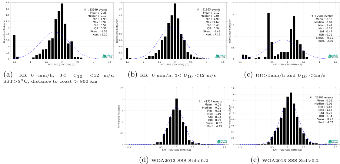
Figure 15: Normalized histogram of \Delta SSS (SMOS SSS L3 v2 - 9-Days (BEC) - TSG (CSIC-UTM)) for 5 different subdatasets corresponding to: RR=0 mm/h, 3 < U_{10} < 12 m/s, SST>5°C, distance to coast > 800 km (a), RR=0 mm/h, 3 < U_{10} < 12 m/s (b), RR>1mm/h and U_{10} < 4 m/s (c), WOA2013 SSS Std<0.2 (d), WOA2013 SSS Std>0.2 (e).
