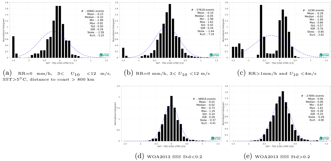
Figure 13: Normalized histogram of \Delta SSS (SMOS SSS L3 v2 - 9-Days (BEC) - TSG (CSIC-UTM)) for 5 different subdatasets corresponding to: RR=0 mm/h, 3 < U_{10} < 12 m/s, SST > 5^\circ C , distance to coast > 800 km (a), RR=0 mm/h, 3 < U_{10} < 12 m/s (b), RR>1mm/h and U_{10} < 4 m/s (c), WOA2013 SSS Std<0.2 (d), WOA2013 SSS Std>0.2 (e).
