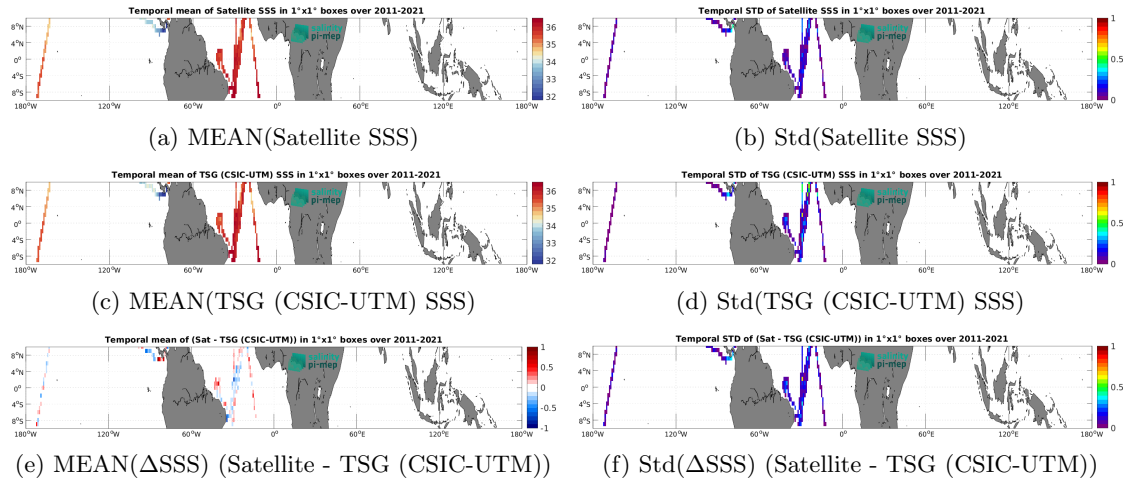
Figure 6: Temporal mean (left) and Std (right) of SSS from SMOS SSS L3 v2 - 9-Days (BEC) (top), TSG (CSIC-UTM) (middle), and of \Delta SSS (Satellite - TSG (CSIC-UTM)). Only match-up pairs are used to generate these maps.
