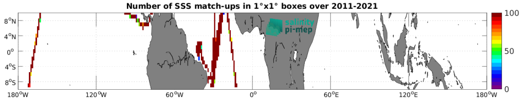
Figure 4: Number of SSS match-ups between TSG (CSIC-UTM) SSS and the SMOS SSS L3 v2 - 9-Days (BEC) SSS product for the Equatorial Ocean 10N-10S Pi-MEP region over 1^\circ \times 1^\circ boxes and for the full satellite product period.
