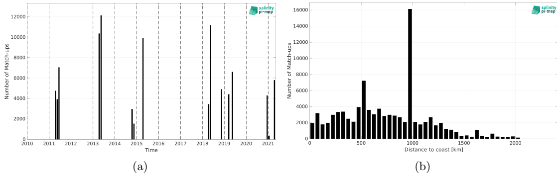
Figure 1: Number of match-ups between TSG (CSIC-UTM) and SMOS SSS L3 v2 - 9-Days (BEC) SSS as a function of time (a) and as function of the distance to coast (b) over the Equatorial Ocean 10N-10S Pi-MEP region and for the full satellite product period.
