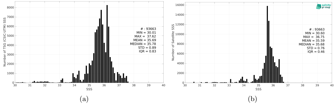
Figure 2: Histograms of SSS from TSG (CSIC-UTM) (a) and SMOS SSS L3 v2 - 9-Days (BEC) (b) considering all match-up pairs per bins of 0.1 over the Equatorial Ocean 10N-10S Pi-MEP region and for the full satellite product period.
