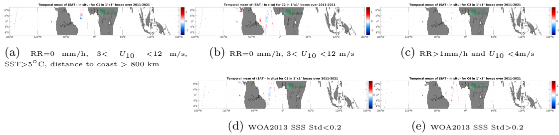
Figure 12: Temporal mean gridded over spatial boxes of size 1^\circ \times 1^\circ of \Delta SSS (SMOS SSS L3 v2 - 9-Days (BEC) - TSG (CSIC-UTM)) for 5 different subdatasets corresponding to: RR=0 mm/h, 3 < U_{10} < 12 m/s, SST>5°C, distance to coast > 800 km (a), RR=0 mm/h, 3 < U_{10} < 12 m/s (b), RR>1mm/h and U_{10} < 4 m/s (c), WOA2013 SSS Std<0.2 (d), WOA2013 SSS Std>0.2 (e).
