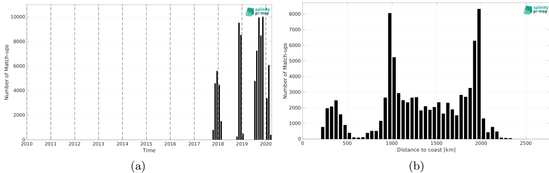
Figure 2: Number of match-ups between Saildrone and SMOS SSS L3 v2 - 9-Days (BEC) SSS as a function of time (a) and as function of the distance to coast (b) over the Equatorial Ocean 10N-10S Pi-MEP region and for the full satellite product period.
