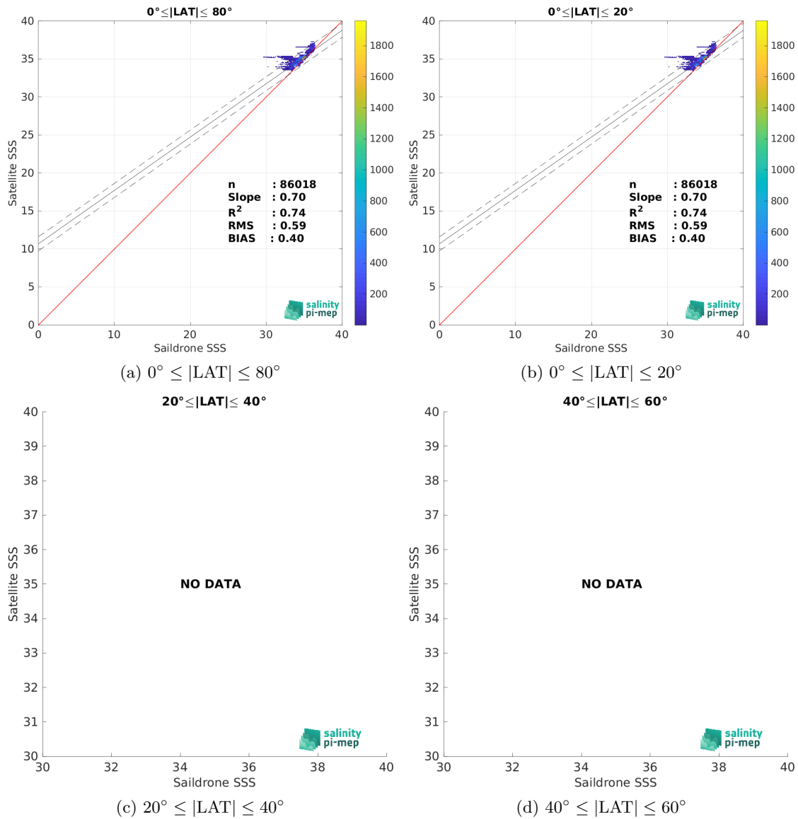
Figure 10: Contour maps of the concentration of SMOS SSS L3 v2 - 9-Days (BEC) SSS (y-axis) versus Sairdrone SSS (x-axis) at match-up pairs for different latitude bands. For each plot, the red line shows x=y . The black thin and dashed lines indicate a linear fit through the data cloud and the \pm 95\% confidence levels, respectively. The number match-up pairs n , the slope and R^2 coefficient of the linear fit, the root mean square (RMS) and the mean bias between satellite and in situ data are indicated for each latitude band in each plots.
