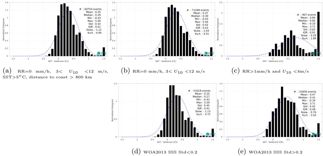
Figure 15: Normalized histogram of \Delta SSS (SMOS SSS L3 v2 - 9-Days (BEC) - Saildrone) for 5 different subdatasets corresponding to: RR=0 mm/h, 3 < U_{10} < 12 m/s, SST>5°C, distance to coast > 800 km (a), RR=0 mm/h, 3 < U_{10} < 12 m/s (b), RR>1mm/h and U_{10} < 4 m/s (c), WOA2013 SSS Std<0.2 (d), WOA2013 SSS Std>0.2 (e).
