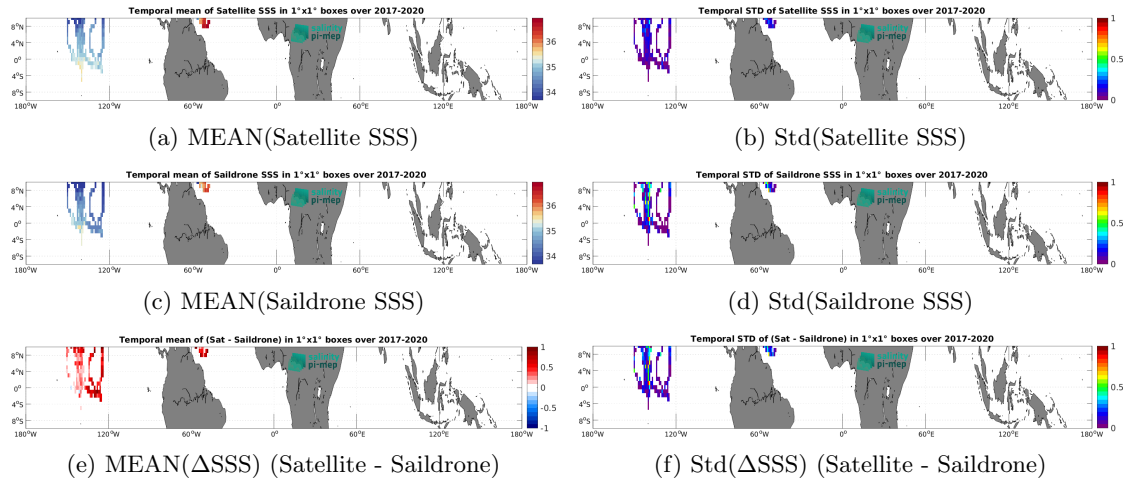
Figure 7: Temporal mean (left) and Std (right) of SSS from SMOS SSS L3 v2 - 9-Days (BEC) (top), Saildrone (middle), and of \Delta SSS (Satellite - Saildrone). Only match-up pairs are used to generate these maps.
