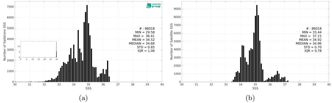
Figure 3: Histograms of SSS from Saildrone (a) and SMOS SSS L3 v2 - 9-Days (BEC) (b) considering all match-up pairs per bins of 0.1 over the Equatorial Ocean 10N-10S Pi-MEP region and for the full satellite product period.
