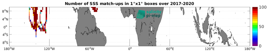
Figure 5: Number of SSS match-ups between Saildrone SSS and the SMOS SSS L3 v2 - 9-Days (BEC) SSS product for the Equatorial Ocean 10N-10S Pi-MEP region over 1^\circ \times 1^\circ boxes and for the full satellite product period.
