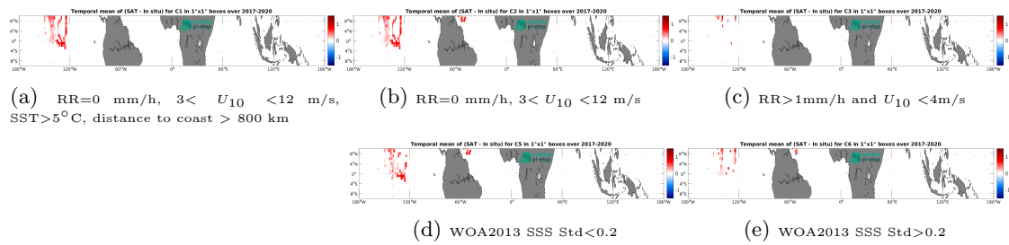
Figure 14: Temporal mean gridded over spatial boxes of size 1^\circ \times 1^\circ of \Delta\text{SSS} (SMOS SSS L3 v2 - 9-Days (BEC) - Saildrone) for 5 different subdatasets corresponding to:RR=0 mm/h, 3 < U_{10} < 12 m/s, SST>5°C, distance to coast > 800 km (a), RR=0 mm/h, 3 < U_{10} < 12 m/s (b), RR>1mm/h and U_{10} < 4 m/s (c), WOA2013 SSS Std<0.2 (d), WOA2013 SSS Std>0.2 (e).
