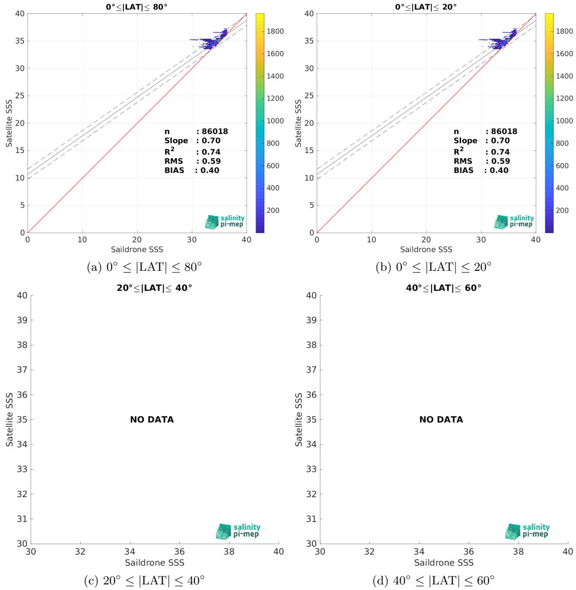
Figure 10: Contour maps of the concentration of SMOS SSS L3 v2 - 9-Days (BEC) SSS (y-axis) versus Sairdrone SSS (x-axis) at match-up pairs for different latitude bands. For each plot, the red line shows x=y . The black thin and dashed lines indicate a linear fit through the data cloud and the \pm 95\% confidence levels, respectively. The number match-up pairs n , the slope and R^2 coefficient of the linear fit, the root mean square (RMS) and the mean bias between satellite and in situ data are indicated for each latitude band in each plots.
