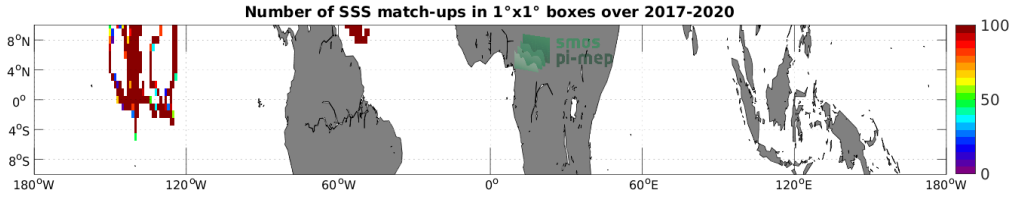
Figure 4: Number of SSS match-ups between Saildrone SSS and the SMOS SSS L3 v2 - 9-Days (BEC) SSS product for the Equatorial Ocean 10N-10S Pi-MEP region over 1^\circ \times 1^\circ boxes and for the full satellite product period.
