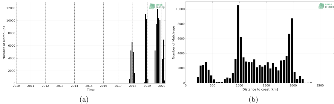
Figure 1: Number of match-ups between Saildrone and SMOS SSS L3 v2 - 9-Days (BEC) SSS as a function of time (a) and as function of the distance to coast (b) over the Equatorial Ocean 10N-10S Pi-MEP region and for the full satellite product period.
