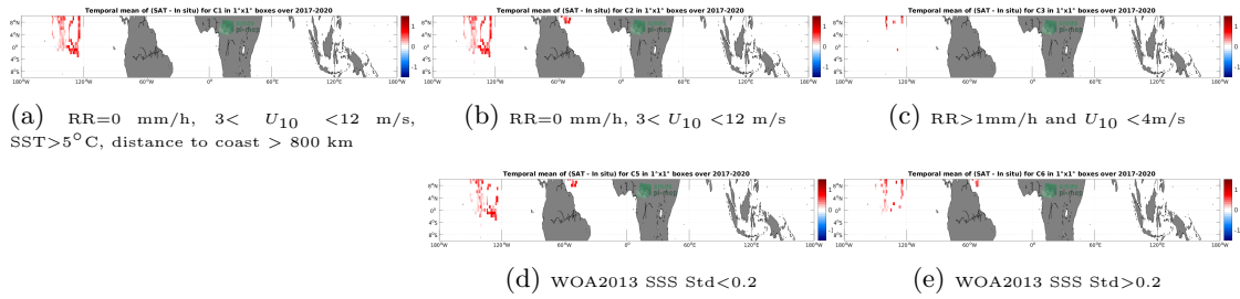
Figure 12: Temporal mean gridded over spatial boxes of size 1^\circ \times 1^\circ of \Delta SSS (SMOS SSS L3 v2 - 9-Days (BEC) - Saildrone) for 5 different subdatasets corresponding to:RR=0 mm/h, 3 < U_{10} < 12 m/s, SST>5°C, distance to coast > 800 km (a), RR=0 mm/h, 3 < U_{10} < 12 m/s (b), RR>1mm/h and U_{10} < 4 m/s (c), WOA2013 SSS Std<0.2 (d), WOA2013 SSS Std>0.2 (e).
