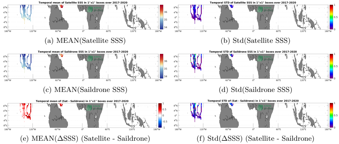
Figure 6: Temporal mean (left) and Std (right) of SSS from SMOS SSS L3 v2 - 9-Days (BEC) (top), Saildrone (middle), and of \Delta SSS (Satellite - Saildrone). Only match-up pairs are used to generate these maps.
