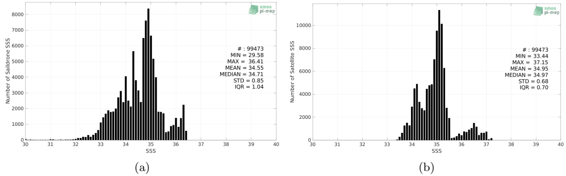
Figure 2: Histograms of SSS from Saildrone (a) and SMOS SSS L3 v2 - 9-Days (BEC) (b) considering all match-up pairs per bins of 0.1 over the Equatorial Ocean 10N-10S Pi-MEP region and for the full satellite product period.
