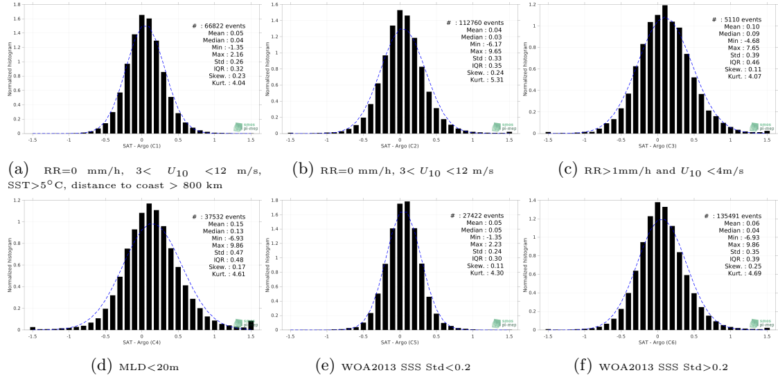
Figure 13: Normalized histogram of \Delta SSS (SMOS SSS L3 v2 - 9-Days (BEC) - Argo) for 6 different subdatasets corresponding to: RR=0 mm/h, 3 < U_{10} < 12 m/s, SST >5^\circ C, distance to coast > 800 km (a), RR=0 mm/h, 3 < U_{10} < 12 m/s (b), RR >1 mm/h and U_{10} < 4 m/s (c), MLD <20 m (d), WOA2013 SSS Std <0.2 (e), WOA2013 SSS Std >0.2 (f).
