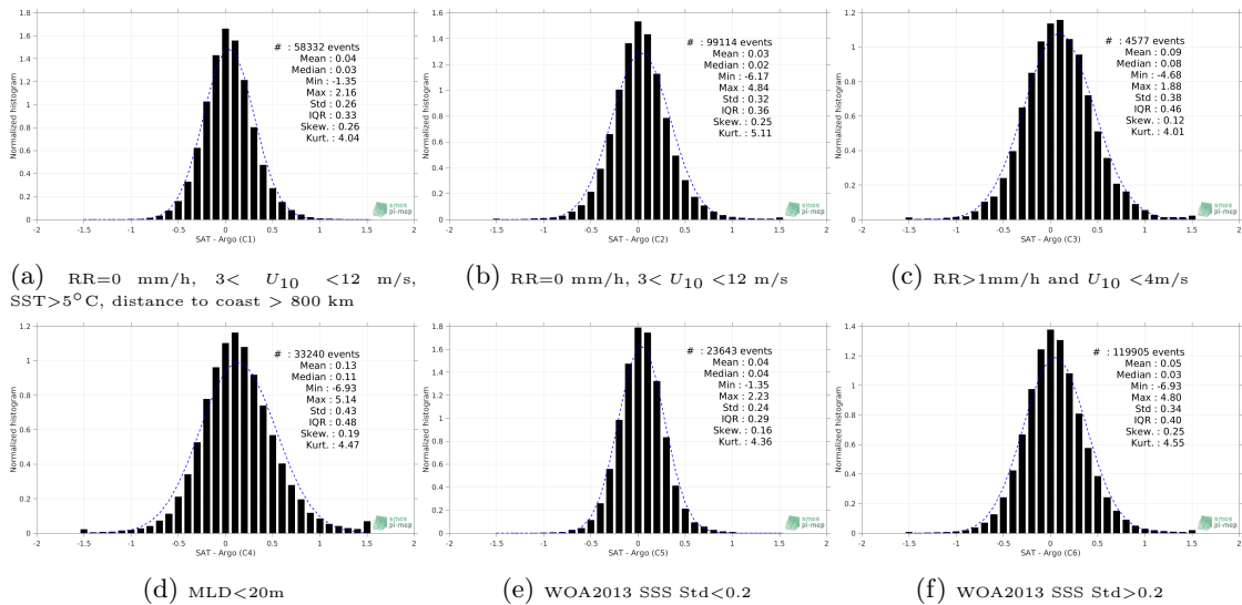
Figure 13: Normalized histogram of \Delta SSS (SMOS SSS L3 v2 - 9-Days (BEC) - Argo) for 6 different subdatasets corresponding to: RR=0 mm/h, 3 < U_{10} < 12 m/s, SST> 5^\circ\text{C} , distance to coast > 800 km (a), RR=0 mm/h, 3 < U_{10} < 12 m/s (b), RR>1mm/h and U_{10} < 4 m/s (c), MLD<20m (d), WOA2013 SSS Std<0.2 (e), WOA2013 SSS Std>0.2 (f).
