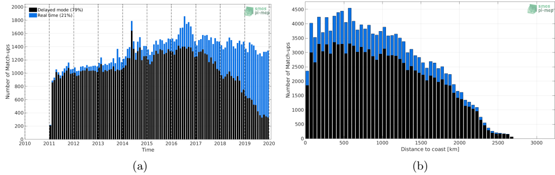
Figure 1: Number of match-ups between Argo and SMOS L3 v2 - 9-Days (BEC) SSS as a function of time (a) and as function of the distance to coast (b) over the Equatorial Ocean 10N-10S Pi-MEP region and for the full satellite product period.
