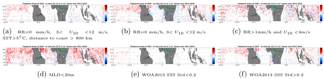
Figure 12: Temporal mean gridded over spatial boxes of size 1°x1° of \Delta SSS (SMOS L3 v2 - 9-Days (BEC) - Argo) for 6 different subdatasets corresponding to:RR=0 mm/h, 3 < U_{10} < 12 m/s, SST>5°C, distance to coast > 800 km (a), RR=0 mm/h, 3 < U_{10} < 12 m/s (b), RR>1mm/h and U_{10} < 4m/s (c),MLD<20m (d),WOA2013 SSS Std<0.2 (e),WOA2013 SSS Std>0.2 (f).
