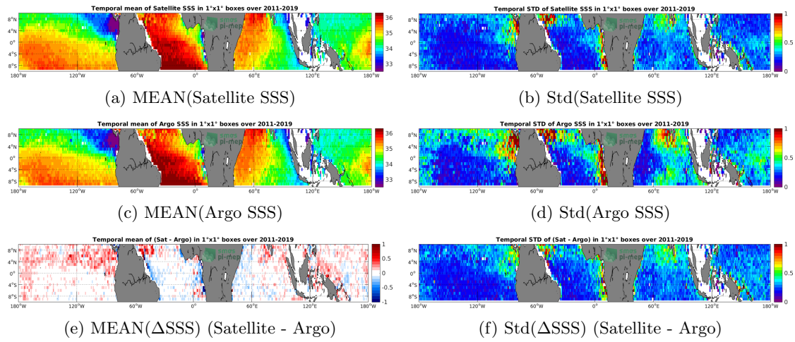
Figure 6: Temporal mean (left) and Std (right) of SSS from SMOS L3 v2 - 9-Days (BEC) (top), Argo (middle), and of \Delta SSS (Satellite - Argo). Only match-up pairs are used to generate these maps.
