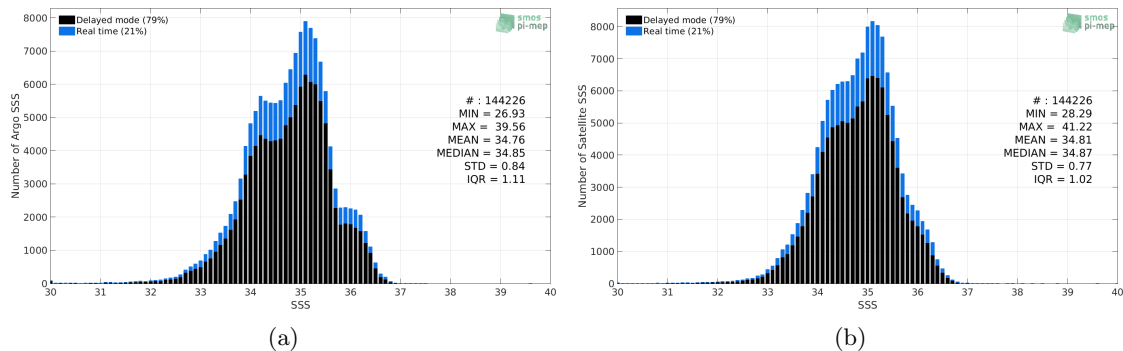
Figure 2: Histograms of SSS from Argo (a) and SMOS L3 v2 - 9-Days (BEC) (b) considering all match-up pairs per bins of 0.1 over the Equatorial Ocean 10N-10S Pi-MEP region and for the full satellite product period.
