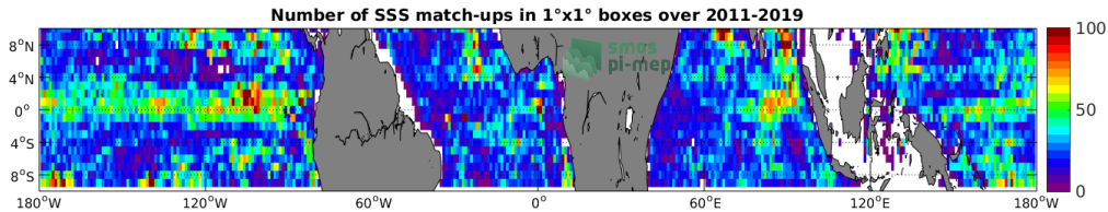
Figure 4: Number of SSS match-ups between Argo SSS and the SMOS L3 v2 - 9-Days (BEC) SSS product for the Equatorial Ocean 10N-10S Pi-MEP region over 1°x1° boxes and for the full satellite product period.
