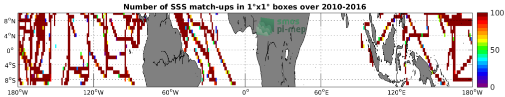
Figure 4: Number of SSS match-ups between TSG-SAMOS SSS and the SMOS-L3-BEC-OA-V1-9DAYS-0.25DEG SSS product for the Equatorial Ocean 10N-10S Pi-MEP region over 1°x1° boxes and for the full satellite product period.
