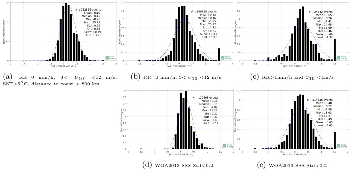
Figure 13: Normalized histogram of ΔSSS (SMOS-L3-BEC-OA-V1-9DAYS-0.25DEG - TSG-SAMOS) for 5 different subdatasets corresponding to: RR=0 mm/h, 3 < U 10 < 12 m/s, SST > 5°C, distance to coast > 800 km (a), RR=0 mm/h, 3 < U 10 < 12 m/s (b), RR > 1mm/h and U 10 < 4m/s (c), WOA2013 SSS Std < 0.2 (d), WOA2013 SSS Std > 0.2 (e).
