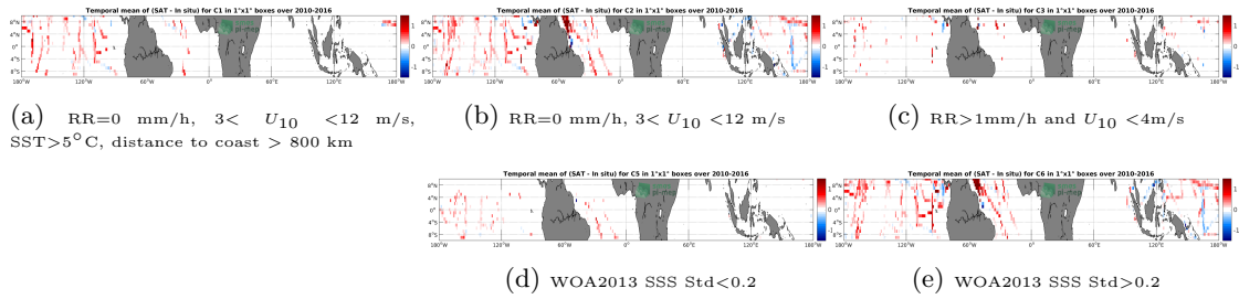
Figure 12: Temporal mean gridded over spatial boxes of size 1^\circ \times 1^\circ of \Delta SSS (SMOS-L3-BEC-OA-V1-9DAYS-0.25DEG - TSG-SAMOS) for 5 different subdatasets corresponding to:RR=0 mm/h, 3 < U_{10} < 12 m/s, SST >5^\circ C, distance to coast > 800 km (a), RR=0 mm/h, 3 < U_{10} < 12 m/s (b), RR >1 mm/h and U_{10} < 4 m/s (c), WOA2013 SSS Std <0.2 (d), WOA2013 SSS Std >0.2 (e).
