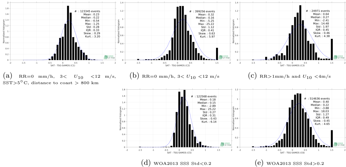
Figure 13: Normalized histogram of \Delta SSS (SMOS-L3-BEC-OA-V1-9DAYS-0.25DEG - TSG-SAMOS) for 5 different subdatasets corresponding to: RR=0 mm/h, 3 < U_{10} < 12 m/s, SST >5^\circ C, distance to coast > 800 km (a), RR=0 mm/h, 3 < U_{10} < 12 m/s (b), RR >1 mm/h and U_{10} < 4 m/s (c), WOA2013 SSS Std <0.2 (d), WOA2013 SSS Std >0.2 (e).
