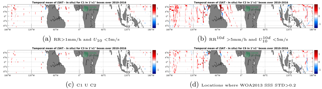
Figure 12: Temporal mean gridded over spatial boxes of size 1^\circ \times 1^\circ of \Delta SSS (SMOS-L3-BEC-OA-V1-9DAYS-0.25DEG - TSG-SAMOS) for 4 different subdatasets corresponding to: RR > 1\text{mm/h} and U_{10} < 5\text{m/s} (a), RR^{10d} > 5\text{mm/h} and U_{10}^{10d} < 5\text{m/s} (b), C1 U C2 (c), Locations where WOA2013 SSS STD > 0.2 (d).
