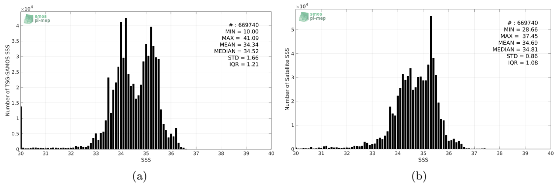
Figure 2: Histograms of SSS from TSG-SAMOS (a) and SMOS-L3-BEC-OA-V1-9DAYS-0.25DEG (b) considering all match-up pairs per bins of 0.1 over the Equatorial Ocean 10N-10S Pi-MEP region and for the full satellite product period.
