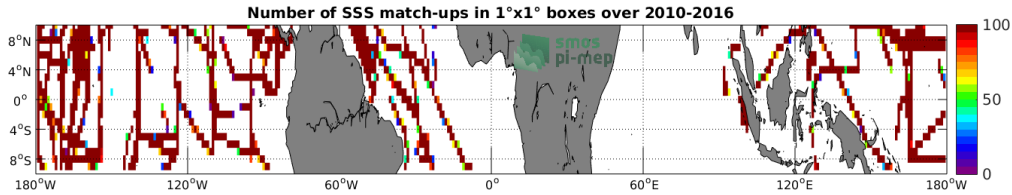
Figure 4: Number of SSS match-ups between TSG-SAMOS SSS and the SMOS-L3-BEC-OA-V1-9DAYS-0.25DEG SSS product for the Equatorial Ocean 10N-10S Pi-MEP region over 1^\circ \times 1^\circ boxes and for the full satellite product period.
