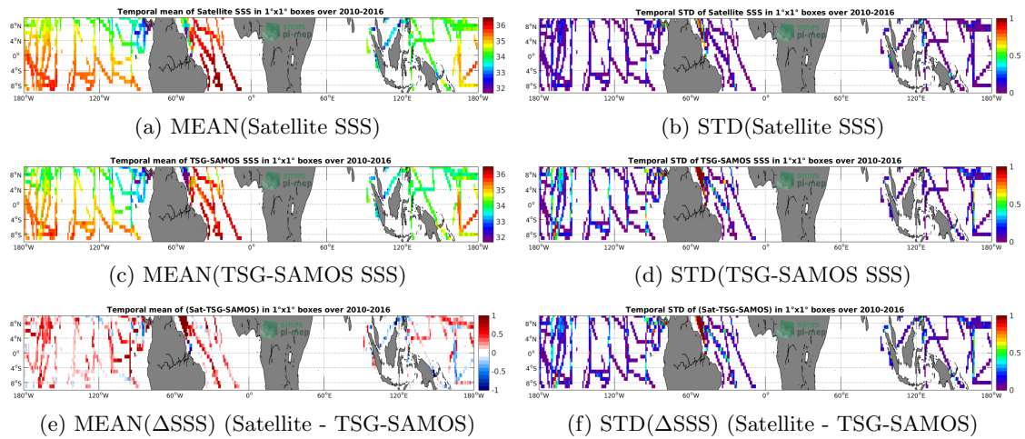
Figure 6: Temporal mean (left) and STD (right) of SSS from SMOS-L3-BEC-OA-V1-9DAYS-0.25DEG (top), TSG-SAMOS (middle), and of \Delta SSS (Satellite - TSG-SAMOS). Only match-up pairs are used to generate these maps.
