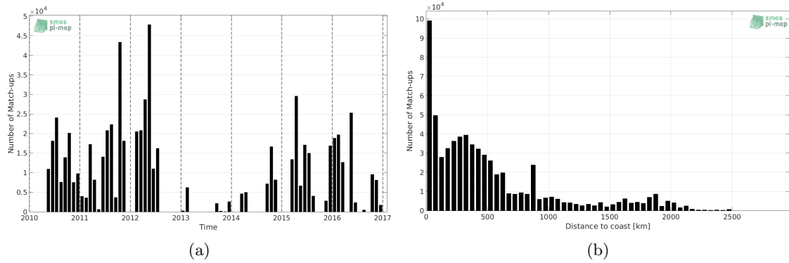
Figure 1: Number of match-ups between TSG-SAMOS and SMOS-L3-BEC-OA-V1-9DAYS-0.25DEG SSS as a function of time (a) and as function of the distance to coast (b) over the Equatorial Ocean 10N-10S Pi-MEP region and for the full satellite product period.
