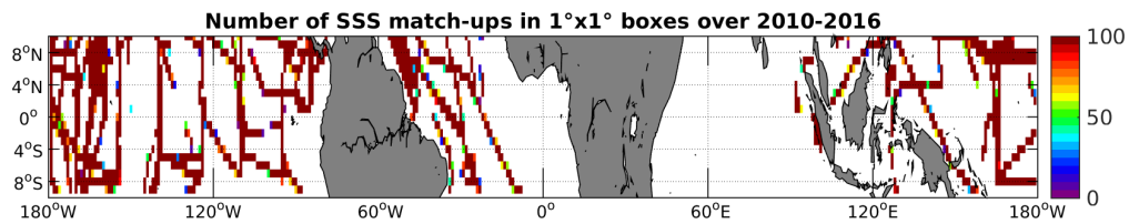
Figure 4: Number of SSS match-ups between TSG-SAMOS SSS and the SMOS-L3-BEC-OA-V1-9DAYS-0.25DEG SSS product for the Equatorial Ocean 10N-10S Pi-MEP region over 1^\circ \times 1^\circ boxes and for the full satellite product period.
