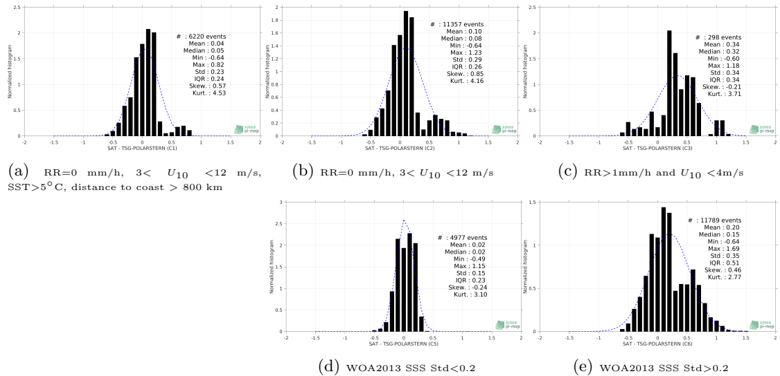
Figure 13: Normalized histogram of \Delta SSS (SMOS-L3-BEC-OA-V1-9DAYS-0.25DEG - TSG-POLARSTERN) for 5 different subdatasets corresponding to: RR=0 mm/h, 3 < U_{10} < 12 m/s, SST >5^\circ C, distance to coast > 800 km (a), RR=0 mm/h, 3 < U_{10} < 12 m/s (b), RR >1 mm/h and U_{10} < 4 m/s (c), WOA2013 SSS Std <0.2 (d), WOA2013 SSS Std >0.2 (e).
