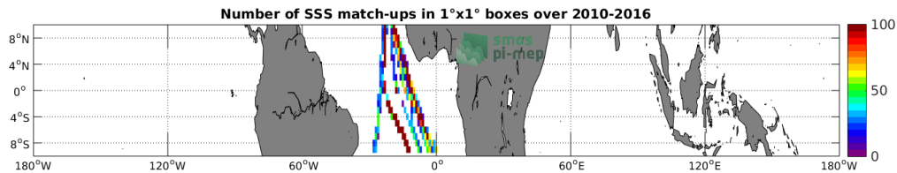
Figure 4: Number of SSS match-ups between TSG-POLARSTERN SSS and the SMOS-L3-BEC-OA-V1-9DAYS-0.25DEG SSS product for the Equatorial Ocean 10N-10S Pi-MEP region over 1^\circ \times 1^\circ boxes and for the full satellite product period.
