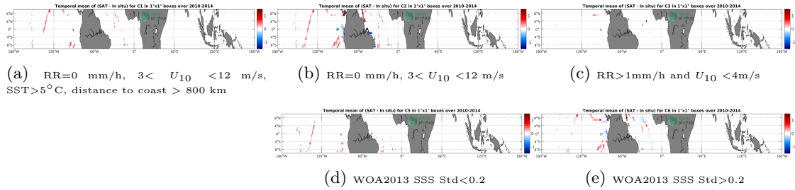
Figure 12: Temporal mean gridded over spatial boxes of size 1^\circ \times 1^\circ of \Delta SSS (SMOS-L3-BEC-OA-V1-9DAYS-0.25DEG - TSG-GOSUD-Sailing-ship) for 5 different subdatasets corresponding to: RR=0 mm/h, 3 < U_{10} < 12 m/s, SST>5°C, distance to coast > 800 km (a), RR=0 mm/h, 3 < U_{10} < 12 m/s (b), RR>1mm/h and U_{10} < 4 m/s (c), WOA2013 SSS Std<0.2 (d), WOA2013 SSS Std>0.2 (e).
