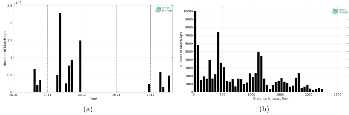
Figure 1: Number of match-ups between TSG-GOSUD-Sailing-ship and SMOS-L3-BEC-OA-V1-9DAYS-0.25DEG SSS as a function of time (a) and as function of the distance to coast (b) over the Equatorial Ocean 10N-10S Pi-MEP region and for the full satellite product period.
