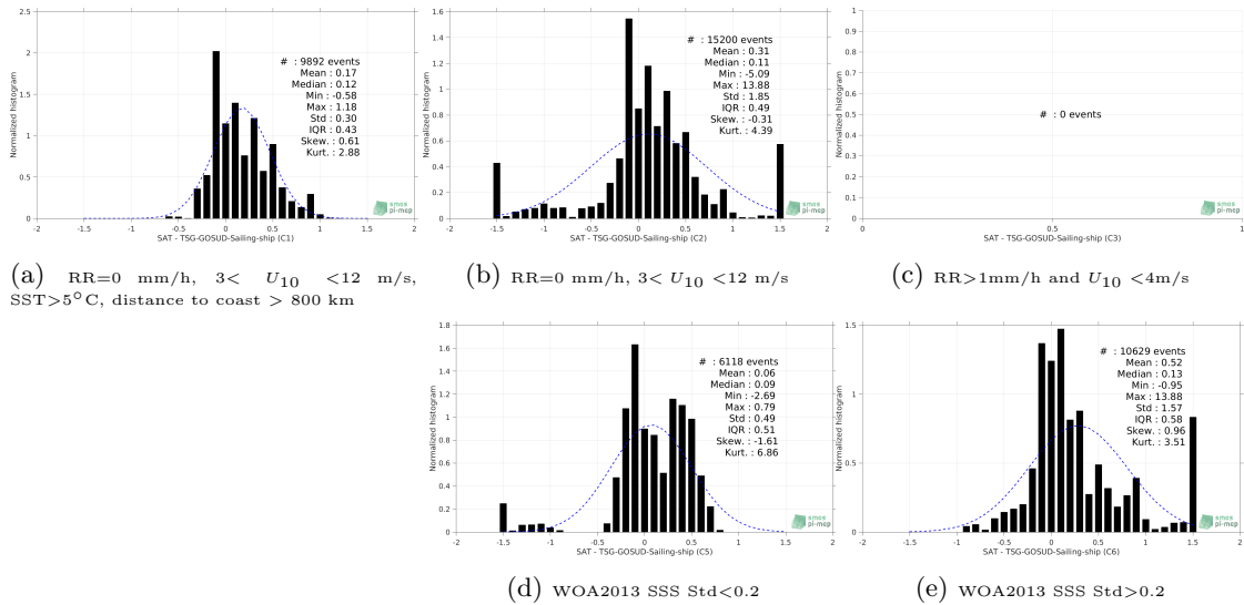
Figure 13: Normalized histogram of \Delta SSS (SMOS-L3-BEC-OA-V1-9DAYS-0.25DEG - TSG-GOSUD-Sailing-ship) for 5 different subdatasets corresponding to: RR=0 mm/h, 3 < U_{10} < 12 m/s, SST >5^\circ C, distance to coast > 800 km (a), RR=0 mm/h, 3 < U_{10} < 12 m/s (b), RR >1 mm/h and U_{10} < 4 m/s (c), WOA2013 SSS Std <0.2 (d), WOA2013 SSS Std >0.2 (e).
