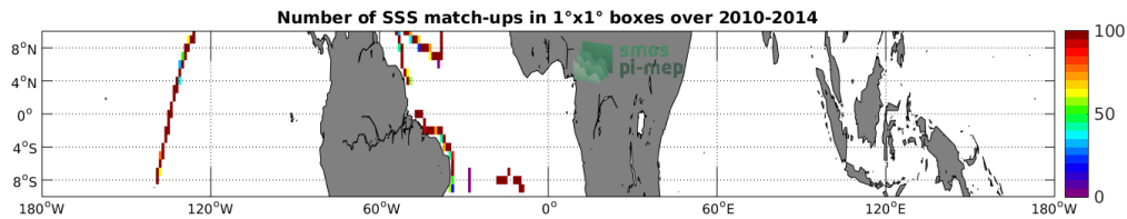
Figure 4: Number of SSS match-ups between TSG-GOSUD-Sailing-ship SSS and the SMOS-L3-BEC-OA-V1-9DAYS-0.25DEG SSS product for the Equatorial Ocean 10N-10S Pi-MEP region over 1°x1° boxes and for the full satellite product period.
