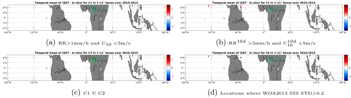
Figure 12: Temporal mean gridded over spatial boxes of size 1^\circ \times 1^\circ of \Delta SSS (SMOS-L3-BEC-OA-V1-9DAYS-0.25DEG - TSG-GOSUD-Sailing-ship) for 4 different subdatasets corresponding to: RR > 1\text{mm/h} and U_{10} < 5\text{m/s} (a), RR^{10d} > 5\text{mm/h} and U_{10}^{10d} < 5\text{m/s} (b), C1 U C2 (c), Locations where WOA2013 SSS STD > 0.2 (d).
