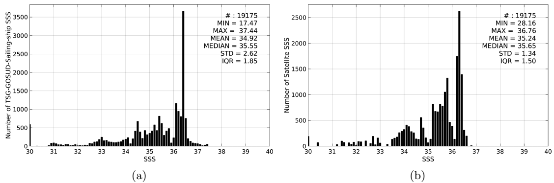
Figure 2: Histograms of SSS from TSG-GOSUD-Sailing-ship (a) and SMOS-L3-BEC-OA-V1-9DAYS-0.25DEG (b) considering all match-up pairs per bins of 0.1 over the Equatorial Ocean 10N-10S Pi-MEP region and for the full satellite product period.
