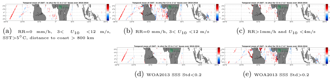
Figure 12: Temporal mean gridded over spatial boxes of size 1°x1° of \Delta SSS (SMOS-L3-BEC-OA-V1-9DAYS-0.25DEG - TSG-GOSUD-Research-vessel) for 5 different subdatasets corresponding to: RR=0 mm/h, 3 < U_{10} < 12 m/s, SST>5°C, distance to coast > 800 km (a), RR=0 mm/h, 3 < U_{10} < 12 m/s (b), RR>1mm/h and U_{10} < 4m/s (c), WOA2013 SSS Std<0.2 (d), WOA2013 SSS Std>0.2 (e).
