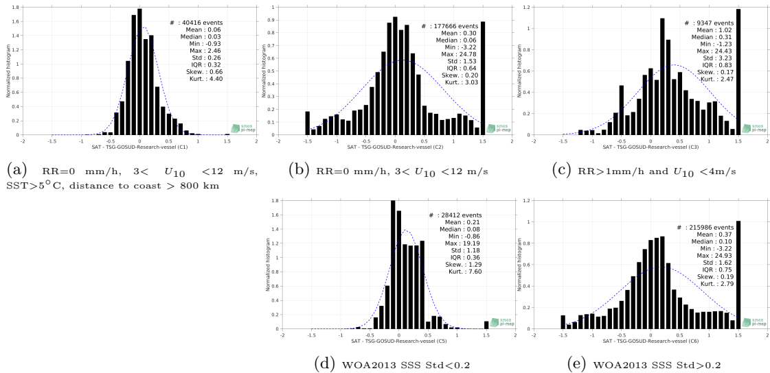
Figure 13: Normalized histogram of \Delta SSS (SMOS-L3-BEC-OA-V1-9DAYS-0.25DEG - TSG-GOSUD-Research-vessel) for 5 different subdatasets corresponding to: RR=0 mm/h, 3 < U_{10} < 12 m/s, SST >5^\circ\text{C} , distance to coast > 800 km (a), RR=0 mm/h, 3 < U_{10} < 12 m/s (b), RR >1 mm/h and U_{10} < 4 m/s (c), WOA2013 SSS Std <0.2 (d), WOA2013 SSS Std >0.2 (e).
