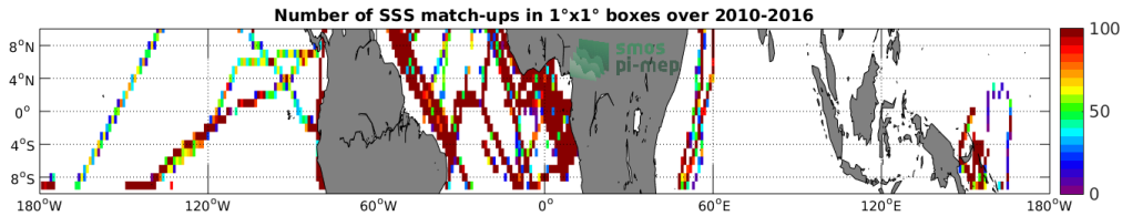
Figure 4: Number of SSS match-ups between TSG-GOSUD-Research-vessel SSS and the SMOS-L3-BEC-OA-V1-9DAYS-0.25DEG SSS product for the Equatorial Ocean 10N-10S Pi-MEP region over 1°x1° boxes and for the full satellite product period.
