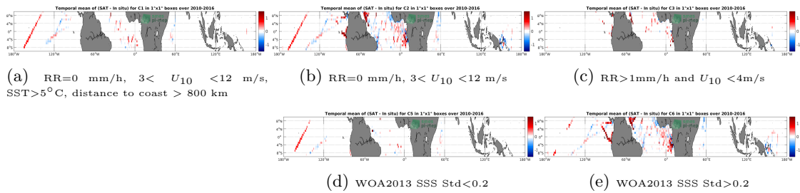
Figure 12: Temporal mean gridded over spatial boxes of size 1^\circ \times 1^\circ of \Delta SSS (SMOS-L3-BEC-OA-V1-9DAYS-0.25DEG - TSG-GOSUD-Research-vessel) for 5 different subdatasets corresponding to: RR=0 mm/h, 3 < U_{10} < 12 m/s, SST >5^\circ\text{C} , distance to coast > 800 km (a), RR=0 mm/h, 3 < U_{10} < 12 m/s (b), RR >1 mm/h and U_{10} < 4 m/s (c), WOA2013 SSS Std <0.2 (d), WOA2013 SSS Std >0.2 (e).
