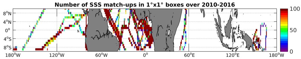
Figure 4: Number of SSS match-ups between TSG-GOSUD-Research-vessel SSS and the SMOS-L3-BEC-OA-V1-9DAYS-0.25DEG SSS product for the Equatorial Ocean 10N-10S Pi-MEP region over 1^\circ \times 1^\circ boxes and for the full satellite product period.
