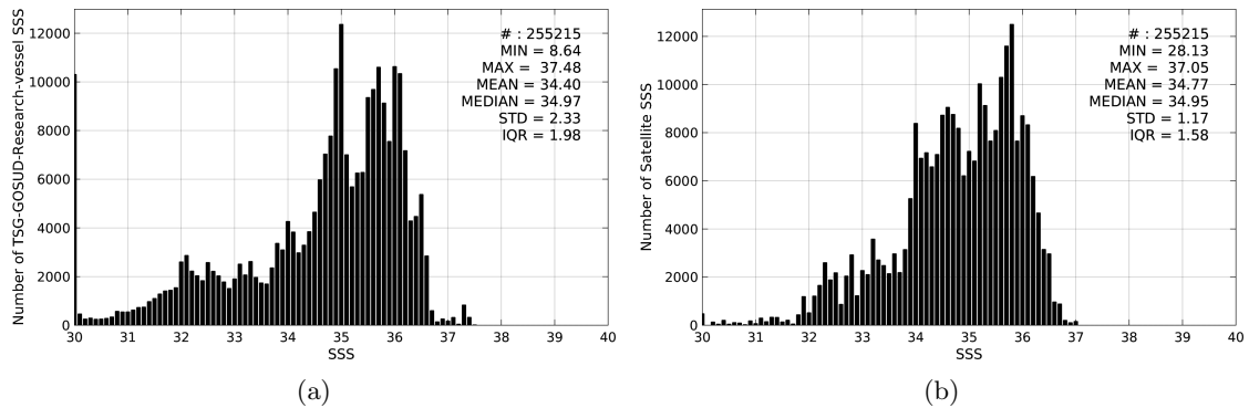
Figure 2: Histograms of SSS from TSG-GOSUD-Research-vessel (a) and SMOS-L3-BEC-OA-V1-9DAYS-0.25DEG (b) considering all match-up pairs per bins of 0.1 over the Equatorial Ocean 10N-10S Pi-MEP region and for the full satellite product period.
