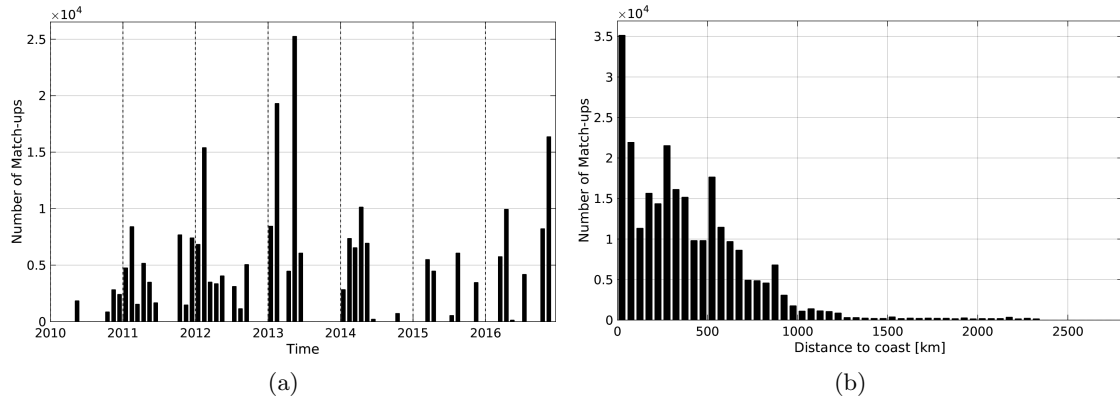
Figure 1: Number of match-ups between TSG-GOSUD-Research-vessel and SMOS-L3-BEC-OA-V1-9DAYS-0.25DEG SSS as a function of time (a) and as function of the distance to coast (b) over the Equatorial Ocean 10N-10S Pi-MEP region and for the full satellite product period.
