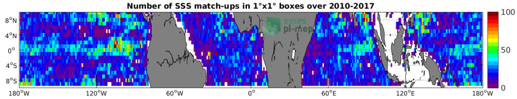
Figure 4: Number of SSS match-ups between Argo SSS and the SMOS-L3-BEC-OA-V1-9DAYS-0.25DEG SSS product for the Equatorial Ocean 10N-10S Pi-MEP region over 1°x1° boxes and for the full satellite product period.
