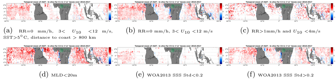
Figure 12: Temporal mean gridded over spatial boxes of size 1^\circ \times 1^\circ of \Delta SSS (SMOS-L3-BEC-OA-V1-9DAYS-0.25DEG - Argo) for 6 different subdatasets corresponding to: RR=0 mm/h, 3 < U_{10} < 12 m/s, SST > 5^\circ C , distance to coast > 800 km (a), RR=0 mm/h, 3 < U_{10} < 12 m/s (b), RR > 1 mm/h and U_{10} < 4 m/s (c), MLD < 20 m (d), WOA2013 SSS Std < 0.2 (e), WOA2013 SSS Std > 0.2 (f).
