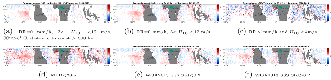
Figure 12: Temporal mean gridded over spatial boxes of size 1^\circ \times 1^\circ of \Delta SSS (SMOS SSS L2-AVERAGED v700 (ESA) - Argo) for 6 different subdatasets corresponding to:RR=0 mm/h, 3 < U_{10} < 12 m/s, SST >5^\circ C, distance to coast > 800 km (a), RR=0 mm/h, 3 < U_{10} < 12 m/s (b), RR >1 mm/h and U_{10} < 4 m/s (c),MLD <20 m (d),WOA2013 SSS Std <0.2 (e),WOA2013 SSS Std >0.2 (f).
