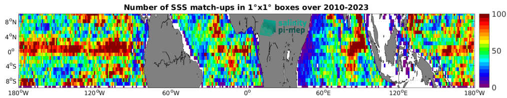
Figure 4: Number of SSS match-ups between Argo SSS and the SMOS SSS L2-AVERAGED v700 (ESA) SSS product for the Equatorial Ocean 10N-10S Pi-MEP region over 1^\circ \times 1^\circ boxes and for the full satellite product period.
