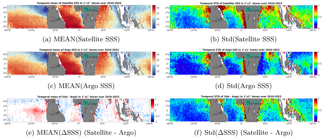
Figure 6: Temporal mean (left) and Std (right) of SSS from SMOS SSS L2-AVERAGED v700 (ESA) (top), Argo (middle), and of \Delta SSS (Satellite - Argo). Only match-up pairs are used to generate these maps.
