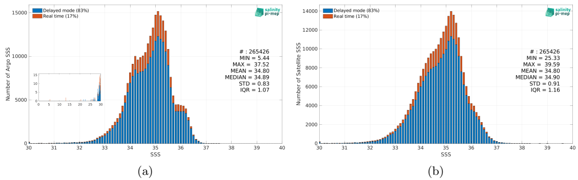
Figure 2: Histograms of SSS from Argo (a) and SMOS SSS L2-AVERAGED v700 (ESA) (b) considering all match-up pairs per bins of 0.1 over the Equatorial Ocean 10N-10S Pi-MEP region and for the full satellite product period.
