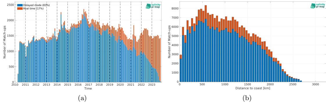
Figure 1: Number of match-ups between Argo and SMOS SSS L2-AVERAGED v700 (ESA) SSS as a function of time (a) and as function of the distance to coast (b) over the Equatorial Ocean 10N-10S Pi-MEP region and for the full satellite product period.
