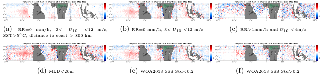
Figure 12: Temporal mean gridded over spatial boxes of size 1^\circ \times 1^\circ of \Delta SSS (SMOS SSS L2-AVERAGED v700 (ESA) - Argo) for 6 different subdatasets corresponding to: RR=0 mm/h, 3 < U_{10} < 12 m/s, SST > 5^\circ C , distance to coast > 800 km (a), RR=0 mm/h, 3 < U_{10} < 12 m/s (b), RR > 1 mm/h and U_{10} < 4 m/s (c), MLD < 20 m (d), WOA2013 SSS Std < 0.2 (e), WOA2013 SSS Std > 0.2 (f).
