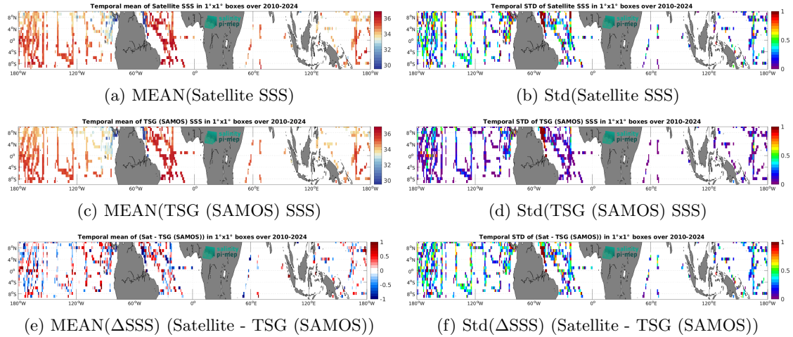
Figure 7: Temporal mean (left) and Std (right) of SSS from SMOS SSS L2 v700 (ESA) (top), TSG (SAMOS) (middle), and of \Delta SSS (Satellite - TSG (SAMOS)). Only match-up pairs are used to generate these maps.
