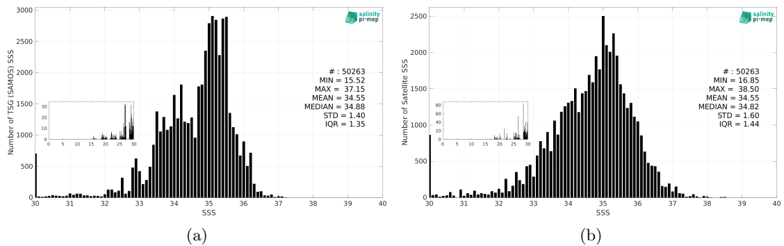
Figure 3: Histograms of SSS from TSG (SAMOS) (a) and SMOS SSS L2 v700 (ESA) (b) considering all match-up pairs per bins of 0.1 over the Equatorial Ocean 10N-10S Pi-MEP region and for the full satellite product period.
