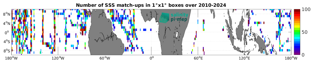
Figure 5: Number of SSS match-ups between TSG (SAMOS) SSS and the SMOS SSS L2 v700 (ESA) SSS product for the Equatorial Ocean 10N-10S Pi-MEP region over 1^\circ \times 1^\circ boxes and for the full satellite product period.
