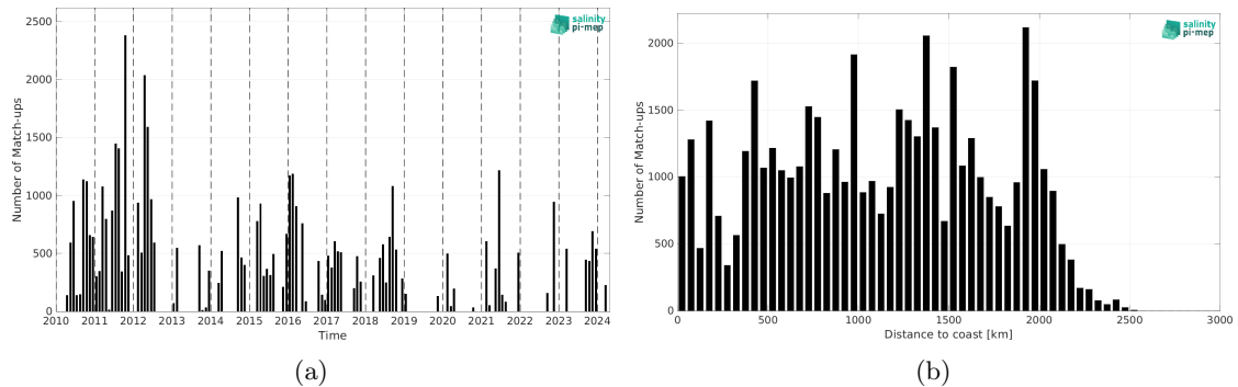
Figure 2: Number of match-ups between TSG (SAMOS) and SMOS SSS L2 v700 (ESA) SSS as a function of time (a) and as function of the distance to coast (b) over the Equatorial Ocean 10N-10S Pi-MEP region and for the full satellite product period.
