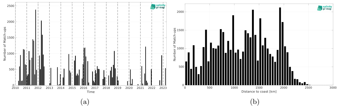
Figure 1: Number of match-ups between TSG (SAMOS) and SMOS SSS L2 v700 (ESA) SSS as a function of time (a) and as function of the distance to coast (b) over the Equatorial Ocean 10N-10S Pi-MEP region and for the full satellite product period.
