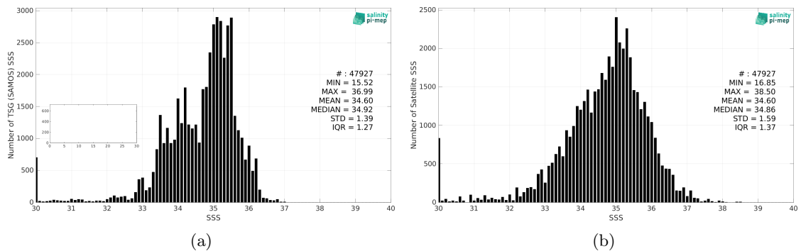
Figure 2: Histograms of SSS from TSG (SAMOS) (a) and SMOS SSS L2 v700 (ESA) (b) considering all match-up pairs per bins of 0.1 over the Equatorial Ocean 10N-10S Pi-MEP region and for the full satellite product period.
