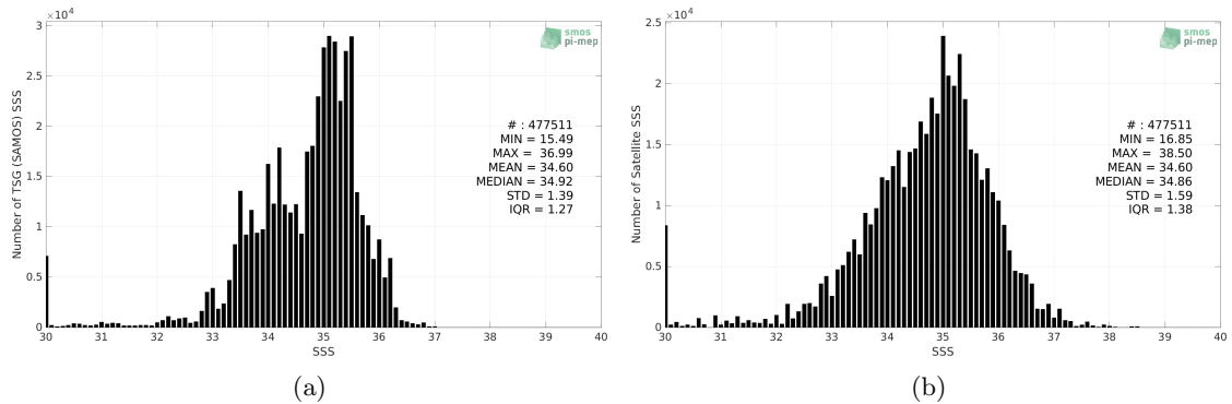
Figure 2: Histograms of SSS from TSG (SAMOS) (a) and SMOS SSS L2 v700 (ESA) (b) considering all match-up pairs per bins of 0.1 over the Equatorial Ocean 10N-10S Pi-MEP region and for the full satellite product period.
