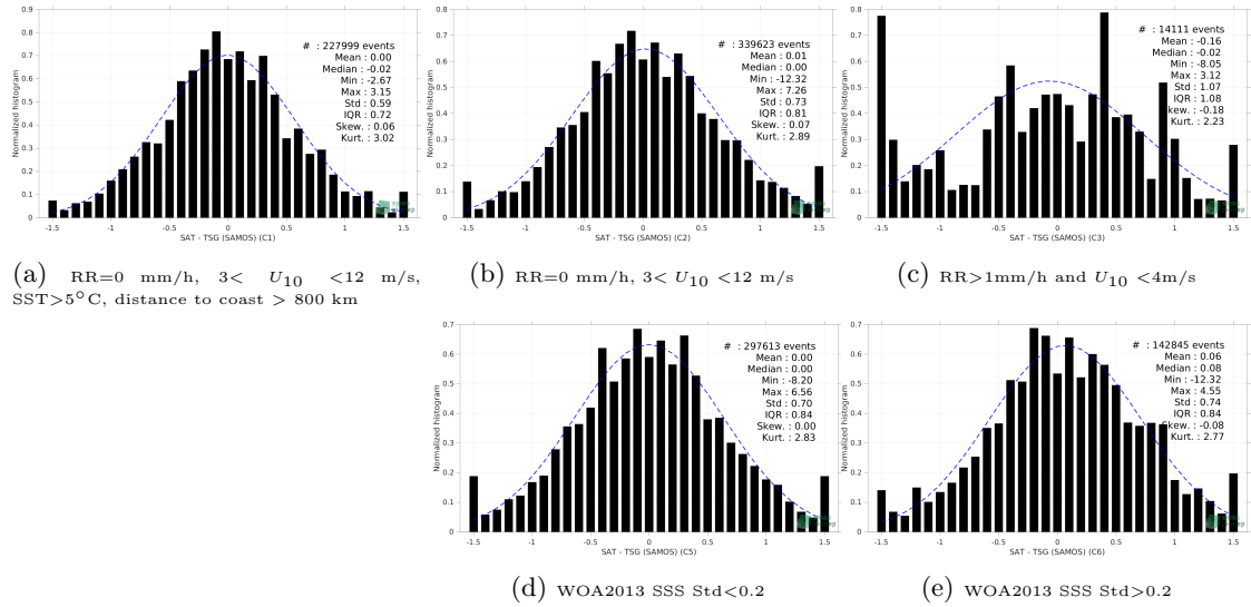
Figure 13: Normalized histogram of \Delta SSS (SMOS SSS L2 v700 (ESA) - TSG (SAMOS)) for 5 different subdatasets corresponding to: RR=0 mm/h, 3 < U_{10} < 12 m/s, SST >5^\circ\text{C} , distance to coast > 800 km (a), RR=0 mm/h, 3 < U_{10} < 12 m/s (b), RR >1 mm/h and U_{10} < 4 m/s (c), WOA2013 SSS Std <0.2 (d), WOA2013 SSS Std >0.2 (e).
