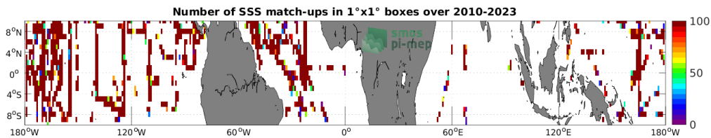
Figure 4: Number of SSS match-ups between TSG (SAMOS) SSS and the SMOS SSS L2 v700 (ESA) SSS product for the Equatorial Ocean 10N-10S Pi-MEP region over 1^\circ \times 1^\circ boxes and for the full satellite product period.
