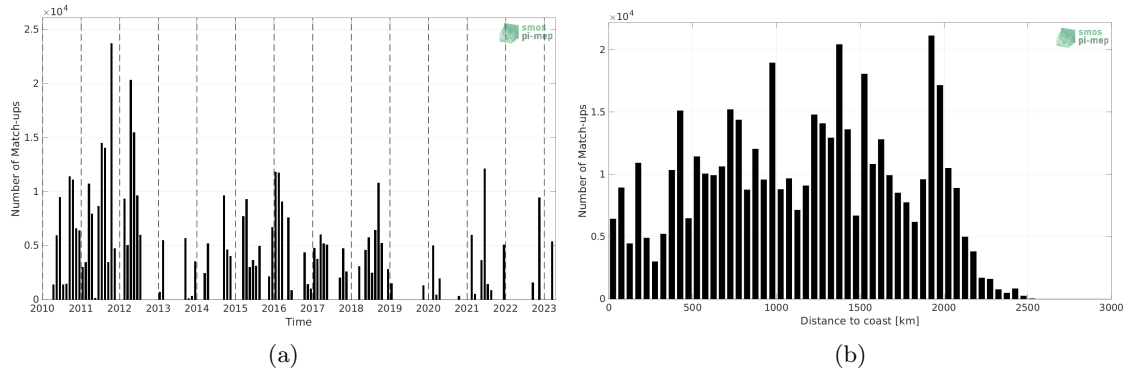
Figure 1: Number of match-ups between TSG (SAMOS) and SMOS SSS L2 v700 (ESA) SSS as a function of time (a) and as function of the distance to coast (b) over the Equatorial Ocean 10N-10S Pi-MEP region and for the full satellite product period.
