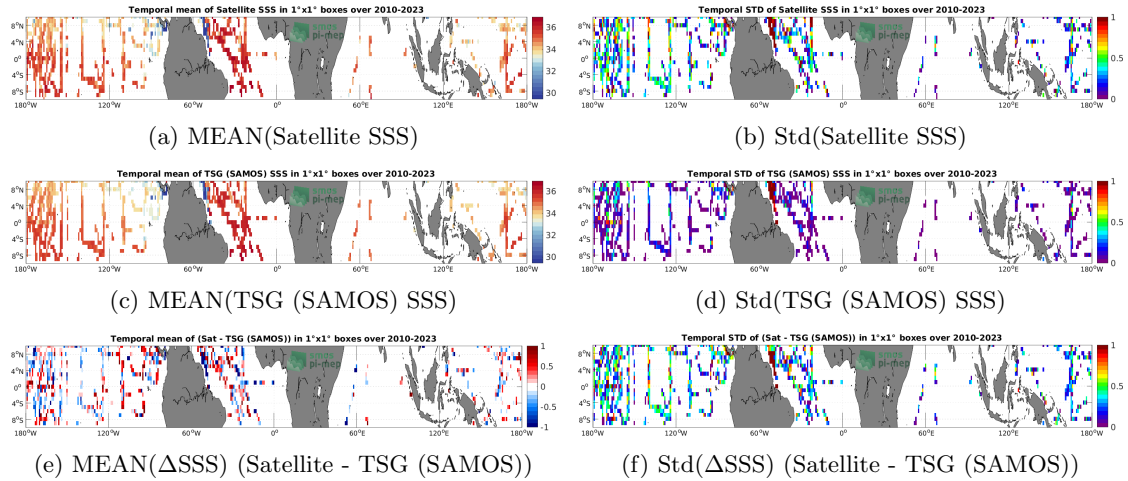
Figure 6: Temporal mean (left) and Std (right) of SSS from SMOS SSS L2 v700 (ESA) (top), TSG (SAMOS) (middle), and of \Delta SSS (Satellite - TSG (SAMOS)). Only match-up pairs are used to generate these maps.
