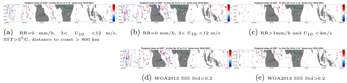
Figure 12: Temporal mean gridded over spatial boxes of size 1^\circ \times 1^\circ of \Delta SSS (SMOS SSS L2 v700 (ESA) - TSG (SAMOS)) for 5 different subdatasets corresponding to:RR=0 mm/h, 3 < U_{10} < 12 m/s, SST >5^\circ\text{C} , distance to coast > 800 km (a), RR=0 mm/h, 3 < U_{10} < 12 m/s (b), RR >1 mm/h and U_{10} < 4 m/s (c), WOA2013 SSS Std <0.2 (d), WOA2013 SSS Std >0.2 (e).
