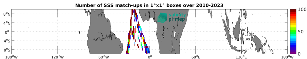
Figure 5: Number of SSS match-ups between TSG (Polarstern) SSS and the SMOS SSS L2 v700 (ESA) SSS product for the Equatorial Ocean 10N-10S Pi-MEP region over 1^\circ \times 1^\circ boxes and for the full satellite product period.
