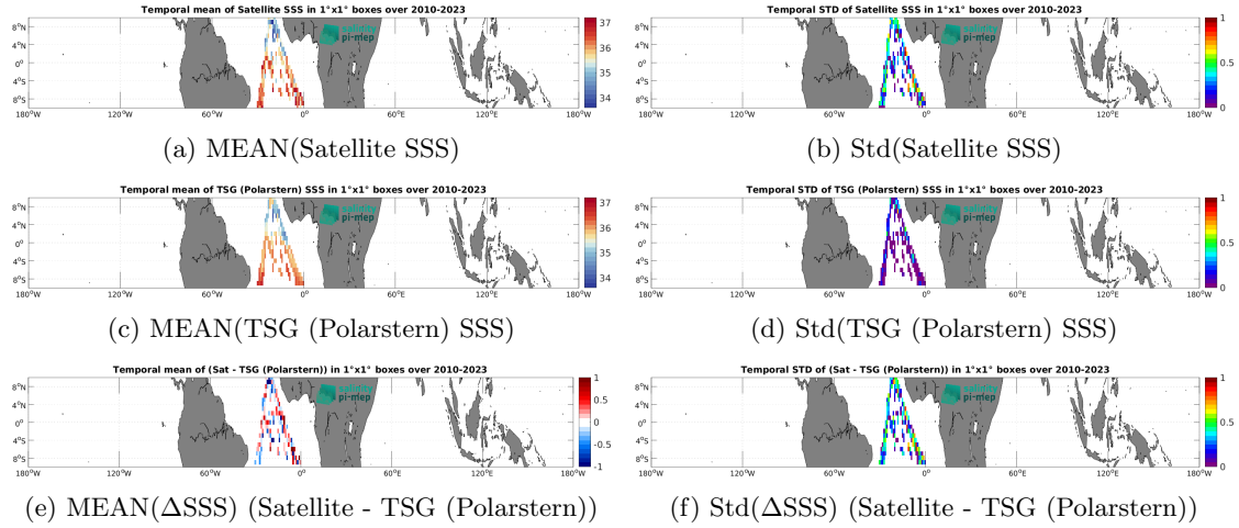
Figure 7: Temporal mean (left) and Std (right) of SSS from SMOS SSS L2 v700 (ESA) (top), TSG (Polarstern) (middle), and of \Delta SSS (Satellite - TSG (Polarstern)). Only match-up pairs are used to generate these maps.
