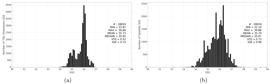
Figure 3: Histograms of SSS from TSG (Polarstern) (a) and SMOS SSS L2 v700 (ESA) (b) considering all match-up pairs per bins of 0.1 over the Equatorial Ocean 10N-10S Pi-MEP region and for the full satellite product period.
