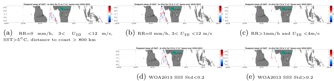
Figure 14: Temporal mean gridded over spatial boxes of size 1^\circ \times 1^\circ of \Delta\text{SSS} (SMOS SSS L2 v700 (ESA) - TSG (Polarstern)) for 5 different subdatasets corresponding to:RR=0 mm/h, 3 < U_{10} < 12 m/s, SST>5°C, distance to coast > 800 km (a), RR=0 mm/h, 3 < U_{10} < 12 m/s (b), RR>1mm/h and U_{10} < 4 m/s (c), WOA2013 SSS Std<0.2 (d), WOA2013 SSS Std>0.2 (e).
