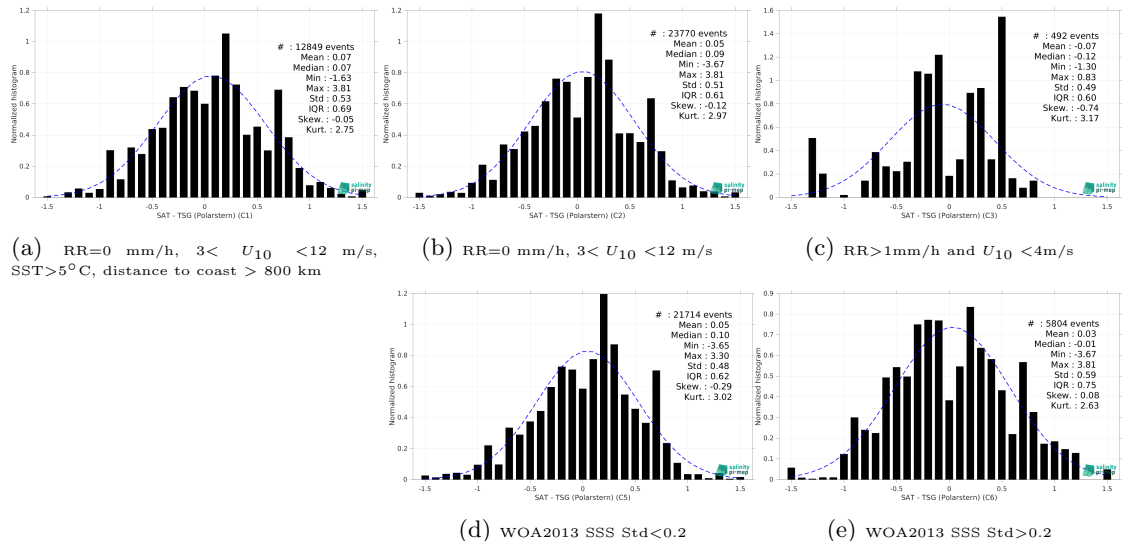
Figure 15: Normalized histogram of \Delta\text{SSS} (SMOS SSS L2 v700 (ESA) - TSG (Polarstern)) for 5 different subdatasets corresponding to: RR=0 mm/h, 3 < U_{10} < 12 m/s, SST>5°C, distance to coast > 800 km (a), RR=0 mm/h, 3 < U_{10} < 12 m/s (b), RR>1mm/h and U_{10} < 4 m/s (c), WOA2013 SSS Std<0.2 (d), WOA2013 SSS Std>0.2 (e).
