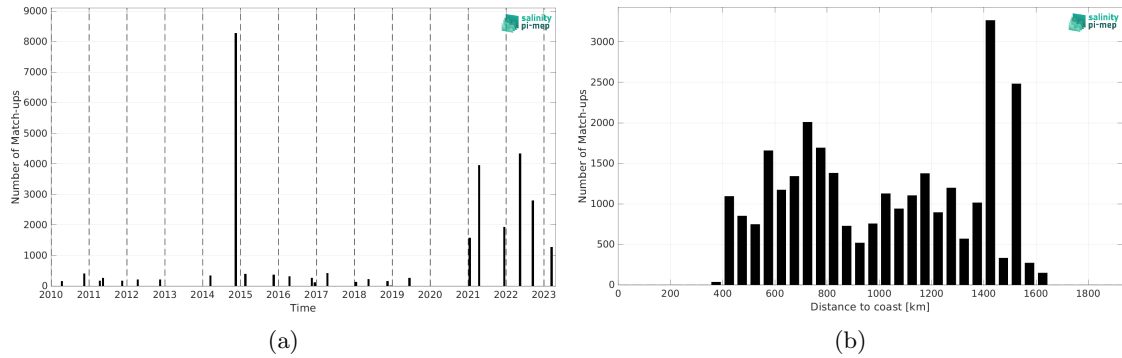
Figure 2: Number of match-ups between TSG (Polarstern) and SMOS SSS L2 v700 (ESA) SSS as a function of time (a) and as function of the distance to coast (b) over the Equatorial Ocean 10N-10S Pi-MEP region and for the full satellite product period.
