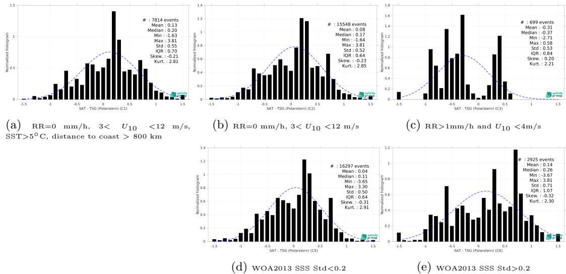
Figure 13: Normalized histogram of \Delta SSS (SMOS SSS L2 v700 (ESA) - TSG (Polarstern)) for 5 different subdatasets corresponding to: RR=0 mm/h, 3 < U_{10} < 12 m/s, SST > 5^\circ C , distance to coast > 800 km (a), RR=0 mm/h, 3 < U_{10} < 12 m/s (b), RR>1mm/h and U_{10} < 4 m/s (c), WOA2013 SSS Std<0.2 (d), WOA2013 SSS Std>0.2 (e).
