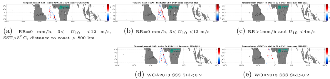
Figure 12: Temporal mean gridded over spatial boxes of size 1^\circ \times 1^\circ of \Delta SSS (SMOS SSS L2 v700 (ESA) - TSG (Polarstern)) for 5 different subdatasets corresponding to:RR=0 mm/h, 3 < U_{10} < 12 m/s, SST > 5^\circ C , distance to coast > 800 km (a), RR=0 mm/h, 3 < U_{10} < 12 m/s (b), RR>1mm/h and U_{10} < 4 m/s (c), WOA2013 SSS Std<0.2 (d), WOA2013 SSS Std>0.2 (e).
