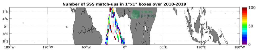
Figure 4: Number of SSS match-ups between TSG (Polarstern) SSS and the SMOS SSS L2 v700 (ESA) SSS product for the Equatorial Ocean 10N-10S Pi-MEP region over 1°×1° boxes and for the full satellite product period.
