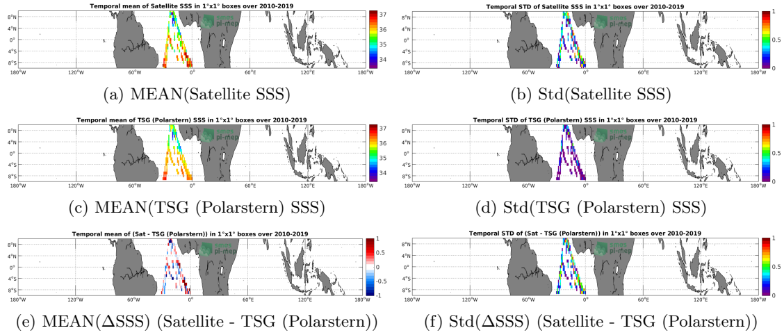
Figure 6: Temporal mean (left) and Std (right) of SSS from SMOS SSS L2 v700 (ESA) (top), TSG (Polarstern) (middle), and of \Delta SSS (Satellite - TSG (Polarstern)). Only match-up pairs are used to generate these maps.
