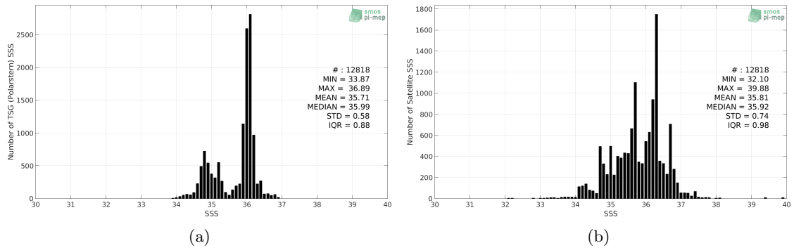
Figure 2: Histograms of SSS from TSG (Polarstern) (a) and SMOS SSS L2 v700 (ESA) (b) considering all match-up pairs per bins of 0.1 over the Equatorial Ocean 10N-10S Pi-MEP region and for the full satellite product period.
