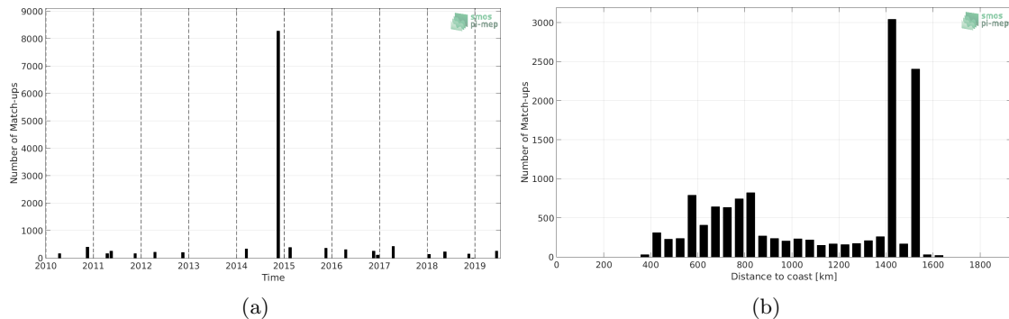
Figure 1: Number of match-ups between TSG (Polarstern) and SMOS SSS L2 v700 (ESA) SSS as a function of time (a) and as function of the distance to coast (b) over the Equatorial Ocean 10N-10S Pi-MEP region and for the full satellite product period.
