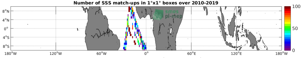
Figure 4: Number of SSS match-ups between TSG (Polarstern) SSS and the SMOS SSS L2 v700 (ESA) SSS product for the Equatorial Ocean 10N-10S Pi-MEP region over 1^\circ \times 1^\circ boxes and for the full satellite product period.
