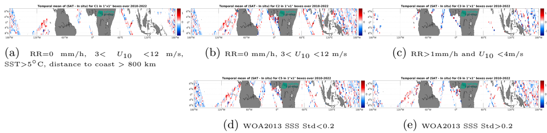
Figure 14: Temporal mean gridded over spatial boxes of size 1^\circ \times 1^\circ of \Delta SSS (SMOS SSS L2 v700 (ESA) - TSG (LEGOS-DM)) for 5 different subdatasets corresponding to: RR=0 mm/h, 3 < U_{10} < 12 m/s, SST>5°C, distance to coast > 800 km (a), RR=0 mm/h, 3 < U_{10} < 12 m/s (b), RR>1mm/h and U_{10} < 4 m/s (c), WOA2013 SSS Std<0.2 (d), WOA2013 SSS Std>0.2 (e).
