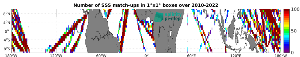
Figure 5: Number of SSS match-ups between TSG (LEGOS-DM) SSS and the SMOS SSS L2 v700 (ESA) SSS product for the Equatorial Ocean 10N-10S Pi-MEP region over 1^\circ \times 1^\circ boxes and for the full satellite product period.
