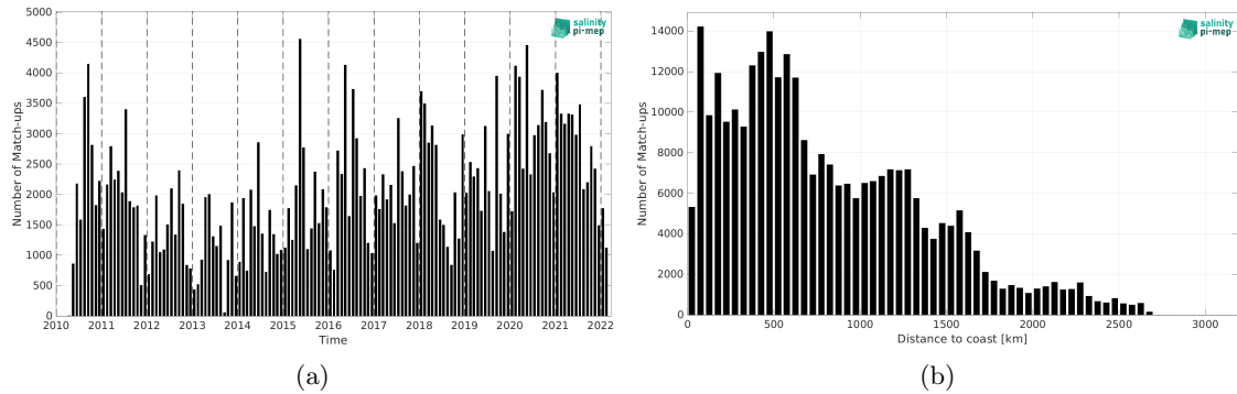
Figure 2: Number of match-ups between TSG (LEGOS-DM) and SMOS SSS L2 v700 (ESA) SSS as a function of time (a) and as function of the distance to coast (b) over the Equatorial Ocean 10N-10S Pi-MEP region and for the full satellite product period.
