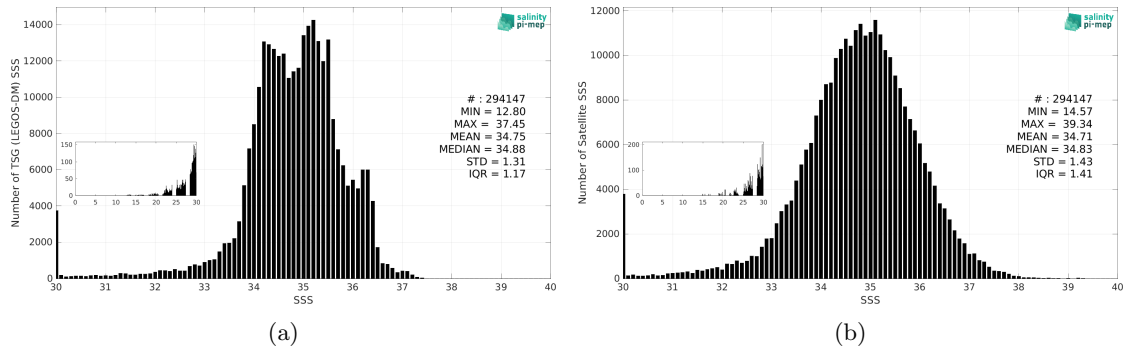
Figure 3: Histograms of SSS from TSG (LEGOS-DM) (a) and SMOS SSS L2 v700 (ESA) (b) considering all match-up pairs per bins of 0.1 over the Equatorial Ocean 10N-10S Pi-MEP region and for the full satellite product period.
