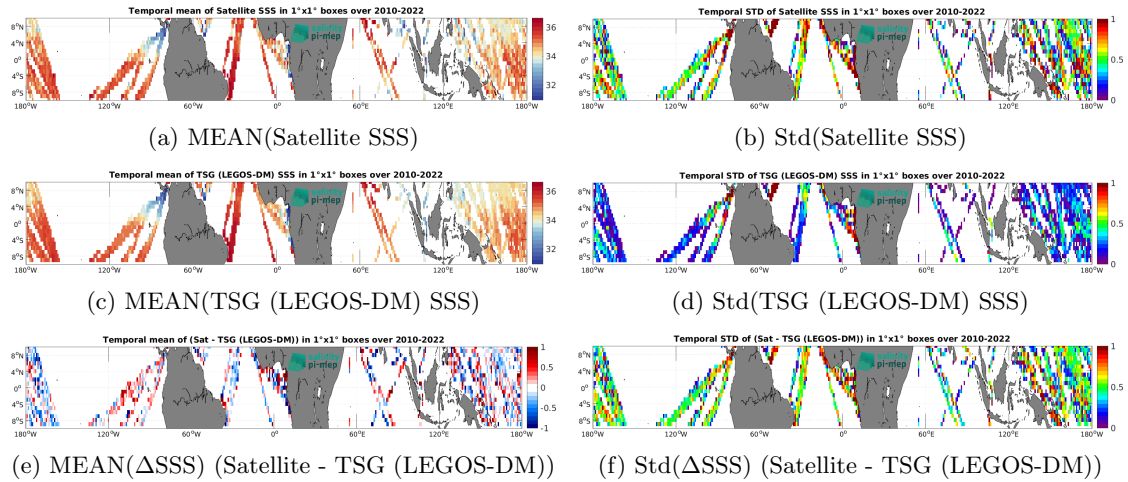
Figure 7: Temporal mean (left) and Std (right) of SSS from SMOS SSS L2 v700 (ESA) (top), TSG (LEGOS-DM) (middle), and of \Delta SSS (Satellite - TSG (LEGOS-DM)). Only match-up pairs are used to generate these maps.
