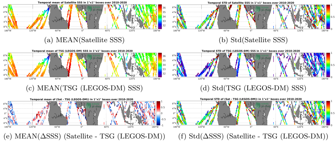
Figure 6: Temporal mean (left) and Std (right) of SSS from SMOS SSS L2 v700 (ESA) (top), TSG (LEGOS-DM) (middle), and of \Delta SSS (Satellite - TSG (LEGOS-DM)). Only match-up pairs are used to generate these maps.
