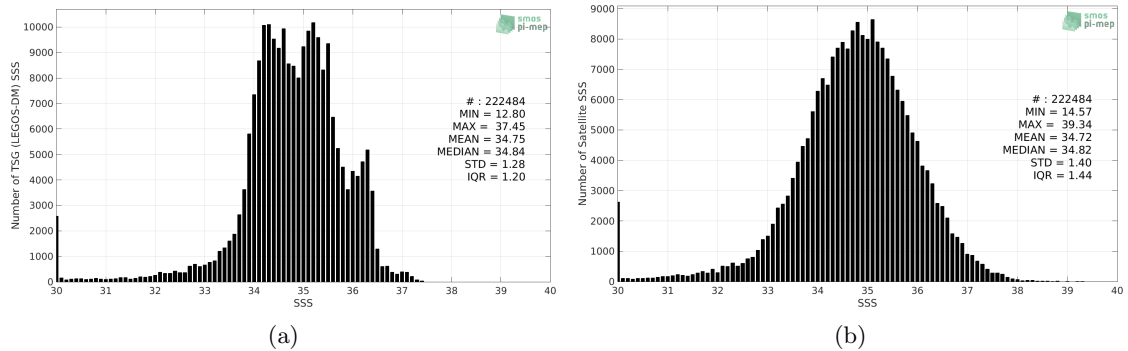
Figure 2: Histograms of SSS from TSG (LEGOS-DM) (a) and SMOS SSS L2 v700 (ESA) (b) considering all match-up pairs per bins of 0.1 over the Equatorial Ocean 10N-10S Pi-MEP region and for the full satellite product period.
