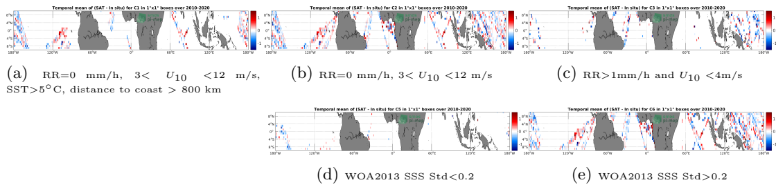
Figure 12: Temporal mean gridded over spatial boxes of size 1^\circ \times 1^\circ of \Delta SSS (SMOS SSS L2 v700 (ESA) - TSG (LEGOS-DM)) for 5 different subdatasets corresponding to:RR=0 mm/h, 3 < U_{10} < 12 m/s, SST > 5^\circ C , distance to coast > 800 km (a), RR=0 mm/h, 3 < U_{10} < 12 m/s (b), RR>1mm/h and U_{10} < 4 m/s (c), WOA2013 SSS Std<0.2 (d), WOA2013 SSS Std>0.2 (e).
