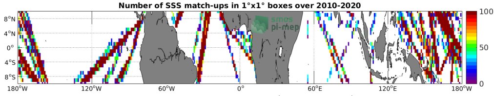
Figure 4: Number of SSS match-ups between TSG (LEGOS-DM) SSS and the SMOS SSS L2 v700 (ESA) SSS product for the Equatorial Ocean 10N-10S Pi-MEP region over 1^\circ \times 1^\circ boxes and for the full satellite product period.
