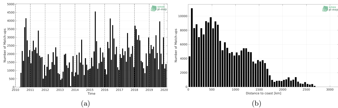
Figure 1: Number of match-ups between TSG (LEGOS-DM) and SMOS SSS L2 v700 (ESA) SSS as a function of time (a) and as function of the distance to coast (b) over the Equatorial Ocean 10N-10S Pi-MEP region and for the full satellite product period.
