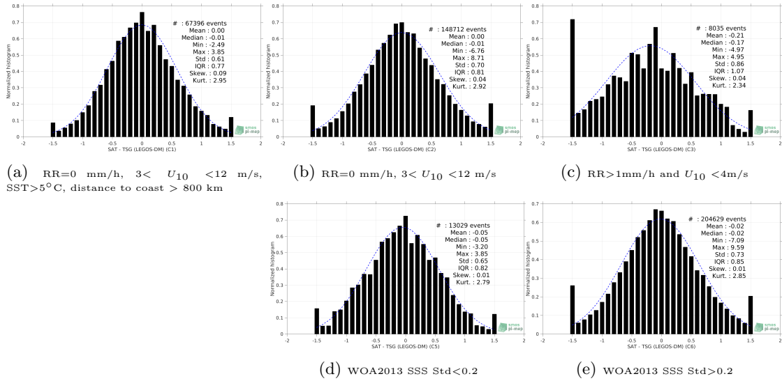
Figure 13: Normalized histogram of \Delta SSS (SMOS SSS L2 v700 (ESA) - TSG (LEGOS-DM)) for 5 different subdatasets corresponding to: RR=0 mm/h, 3 < U_{10} < 12 m/s, SST > 5^\circ C , distance to coast > 800 km (a), RR=0 mm/h, 3 < U_{10} < 12 m/s (b), RR>1mm/h and U_{10} < 4 m/s (c), WOA2013 SSS Std<0.2 (d), WOA2013 SSS Std>0.2 (e).
