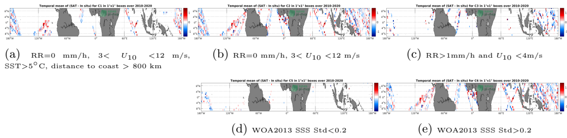
Figure 12: Temporal mean gridded over spatial boxes of size 1°x1° of ΔSSS (SMOS SSS L2 v700 (ESA) - TSG (LEGOS-DM)) for 5 different subdatasets corresponding to:RR=0 mm/h, 3 < U 10 < 12 m/s, SST>5°C, distance to coast > 800 km (a), RR=0 mm/h, 3 < U 10 < 12 m/s (b), RR>1mm/h and U 10 < 4m/s (c), WOA2013 SSS Std<0.2 (d), WOA2013 SSS Std>0.2 (e).
