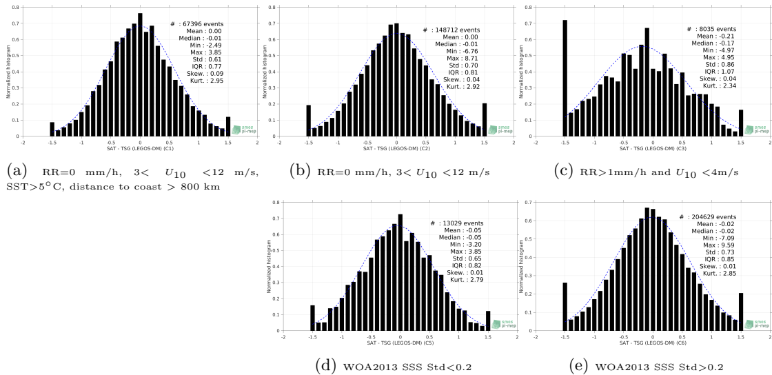
Figure 13: Normalized histogram of ΔSSS (SMOS SSS L2 v700 (ESA) - TSG (LEGOS-DM)) for 5 different subdatasets corresponding to: RR=0 mm/h, 3 < U 10 < 12 m/s, SST>5°C, distance to coast > 800 km (a), RR=0 mm/h, 3 < U 10 < 12 m/s (b), RR>1mm/h and U 10 < 4m/s (c), WOA2013 SSS Std<0.2 (d), WOA2013 SSS Std>0.2 (e).
