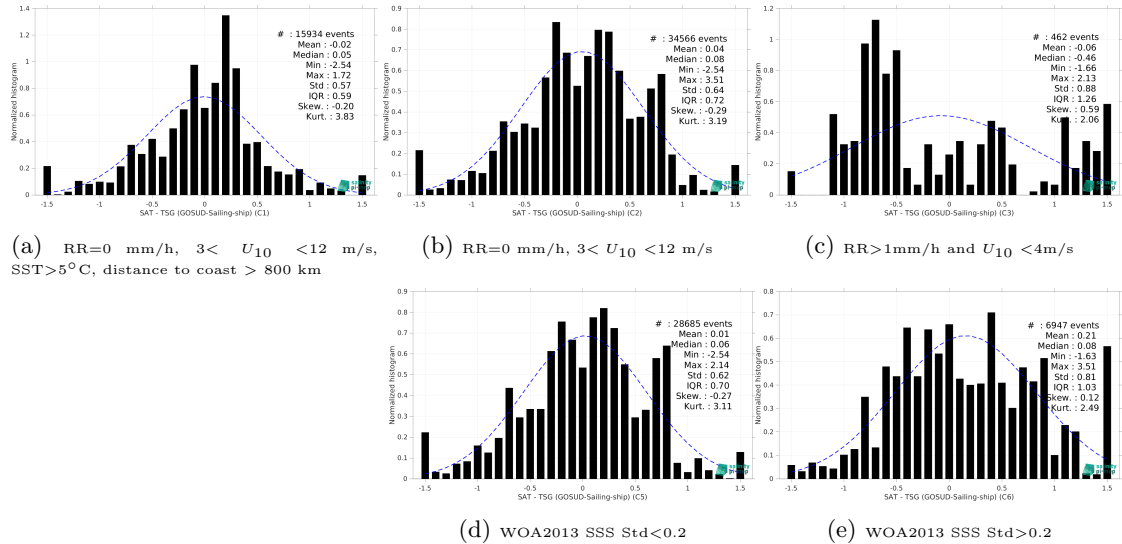
Figure 15: Normalized histogram of \Delta SSS (SMOS SSS L2 v700 (ESA) - TSG (GOSUD-Sailing-ship)) for 5 different subdatasets corresponding to: RR=0 mm/h, 3 < U_{10} < 12 m/s, SST >5^\circ\text{C} , distance to coast > 800 km (a), RR=0 mm/h, 3 < U_{10} < 12 m/s (b), RR >1 mm/h and U_{10} < 4 m/s (c), WOA2013 SSS Std <0.2 (d), WOA2013 SSS Std >0.2 (e).
