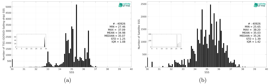
Figure 3: Histograms of SSS from TSG (GOSUD-Sailing-ship) (a) and SMOS SSS L2 v700 (ESA) (b) considering all match-up pairs per bins of 0.1 over the Equatorial Ocean 10N-10S Pi-MEP region and for the full satellite product period.
