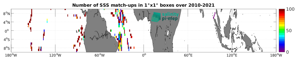
Figure 5: Number of SSS match-ups between TSG (GOSUD-Sailing-ship) SSS and the SMOS SSS L2 v700 (ESA) SSS product for the Equatorial Ocean 10N-10S Pi-MEP region over 1^\circ \times 1^\circ boxes and for the full satellite product period.
