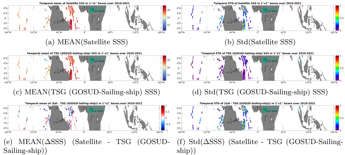
Figure 7: Temporal mean (left) and Std (right) of SSS from SMOS SSS L2 v700 (ESA) (top), TSG (GOSUD-Sailing-ship) (middle), and of \Delta SSS (Satellite - TSG (GOSUD-Sailing-ship)). Only match-up pairs are used to generate these maps.
