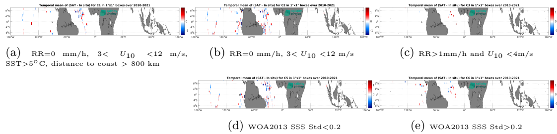
Figure 14: Temporal mean gridded over spatial boxes of size 1^\circ \times 1^\circ of \Delta SSS (SMOS SSS L2 v700 (ESA) - TSG (GOSUD-Sailing-ship)) for 5 different subdatasets corresponding to:RR=0 mm/h, 3 < U_{10} < 12 m/s, SST>5°C, distance to coast > 800 km (a), RR=0 mm/h, 3 < U_{10} < 12 m/s (b), RR>1mm/h and U_{10} < 4 m/s (c), WOA2013 SSS Std<0.2 (d), WOA2013 SSS Std>0.2 (e).
