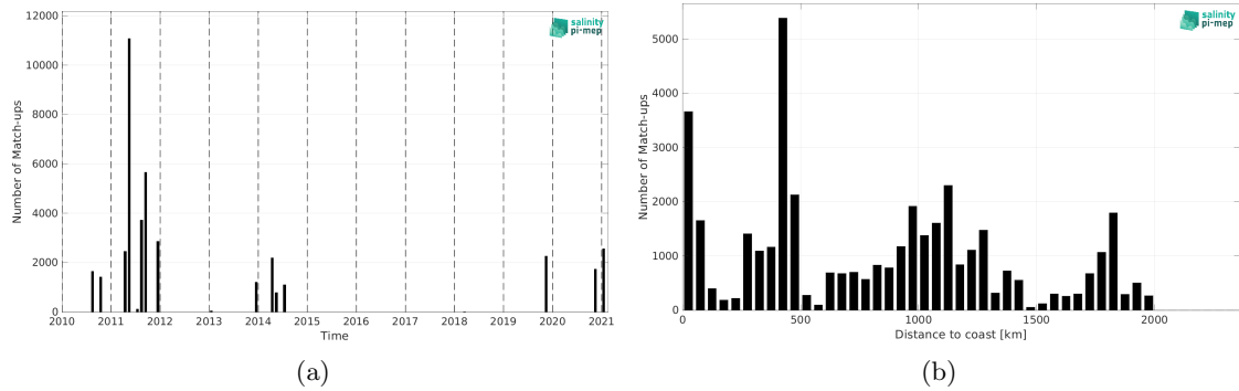
Figure 2: Number of match-ups between TSG (GOSUD-Sailing-ship) and SMOS SSS L2 v700 (ESA) SSS as a function of time (a) and as function of the distance to coast (b) over the Equatorial Ocean 10N-10S Pi-MEP region and for the full satellite product period.
