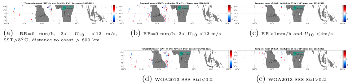
Figure 12: Temporal mean gridded over spatial boxes of size 1^\circ \times 1^\circ of \Delta\text{SSS} (SMOS SSS L2 v700 (ESA) - TSG (GOSUD-Sailing-ship)) for 5 different subdatasets corresponding to:RR=0 mm/h, 3 < U_{10} < 12 m/s, SST>5°C, distance to coast > 800 km (a), RR=0 mm/h, 3 < U_{10} < 12 m/s (b), RR>1mm/h and U_{10} < 4 m/s (c), WOA2013 SSS Std<0.2 (d), WOA2013 SSS Std>0.2 (e).
