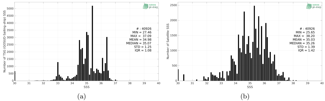
Figure 2: Histograms of SSS from TSG (GOSUD-Sailing-ship) (a) and SMOS SSS L2 v700 (ESA) (b) considering all match-up pairs per bins of 0.1 over the Equatorial Ocean 10N-10S Pi-MEP region and for the full satellite product period.
