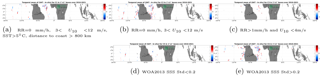
Figure 12: Temporal mean gridded over spatial boxes of size 1^\circ \times 1^\circ of \Delta SSS (SMOS SSS L2 v700 (ESA) - TSG (GOSUD-Sailing-ship)) for 5 different subdatasets corresponding to: RR=0 mm/h, 3 < U_{10} < 12 m/s, SST>5°C, distance to coast > 800 km (a), RR=0 mm/h, 3 < U_{10} < 12 m/s (b), RR>1mm/h and U_{10} < 4 m/s (c), WOA2013 SSS Std<0.2 (d), WOA2013 SSS Std>0.2 (e).
