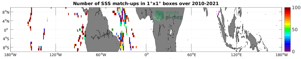
Figure 4: Number of SSS match-ups between TSG (GOSUD-Sailing-ship) SSS and the SMOS SSS L2 v700 (ESA) SSS product for the Equatorial Ocean 10N-10S Pi-MEP region over 1^\circ \times 1^\circ boxes and for the full satellite product period.
