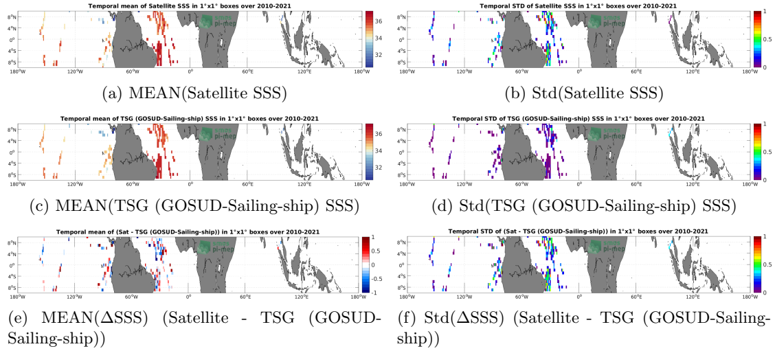
Figure 6: Temporal mean (left) and Std (right) of SSS from SMOS SSS L2 v700 (ESA) (top), TSG (GOSUD-Sailing-ship) (middle), and of \Delta SSS (Satellite - TSG (GOSUD-Sailing-ship)). Only match-up pairs are used to generate these maps.
