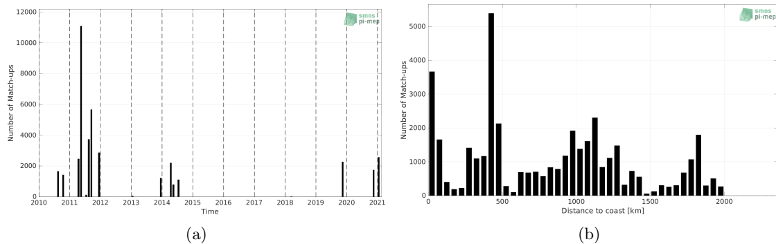
Figure 1: Number of match-ups between TSG (GOSUD-Sailing-ship) and SMOS SSS L2 v700 (ESA) SSS as a function of time (a) and as function of the distance to coast (b) over the Equatorial Ocean 10N-10S Pi-MEP region and for the full satellite product period.
