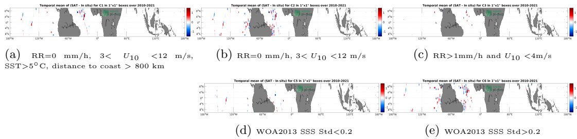
Figure 12: Temporal mean gridded over spatial boxes of size 1^\circ \times 1^\circ of \Delta SSS (SMOS SSS L2 v700 (ESA) - TSG (GOSUD-Sailing-ship)) for 5 different subdatasets corresponding to: RR=0 mm/h, 3 < U_{10} < 12 m/s, SST>5°C, distance to coast > 800 km (a), RR=0 mm/h, 3 < U_{10} < 12 m/s (b), RR>1mm/h and U_{10} < 4 m/s (c), WOA2013 SSS Std<0.2 (d), WOA2013 SSS Std>0.2 (e).
