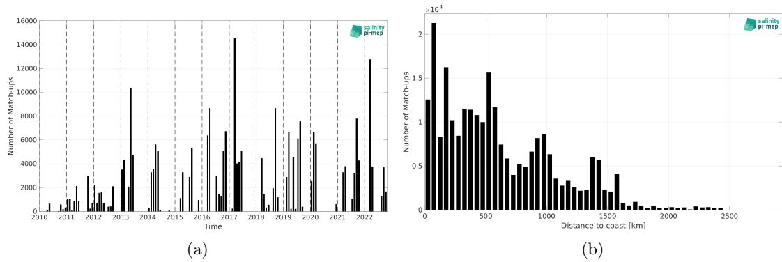
Figure 2: Number of match-ups between TSG (GOSUD-Research-vessel) and SMOS SSS L2 v700 (ESA) SSS as a function of time (a) and as function of the distance to coast (b) over the Equatorial Ocean 10N-10S Pi-MEP region and for the full satellite product period.
