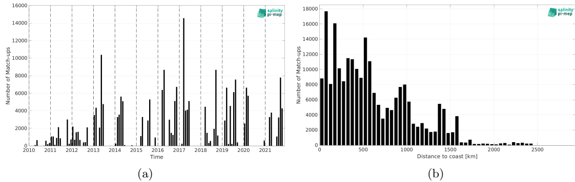
Figure 2: Number of match-ups between TSG (GOSUD-Research-vessel) and SMOS SSS L2 v700 (ESA) SSS as a function of time (a) and as function of the distance to coast (b) over the Equatorial Ocean 10N-10S Pi-MEP region and for the full satellite product period.
