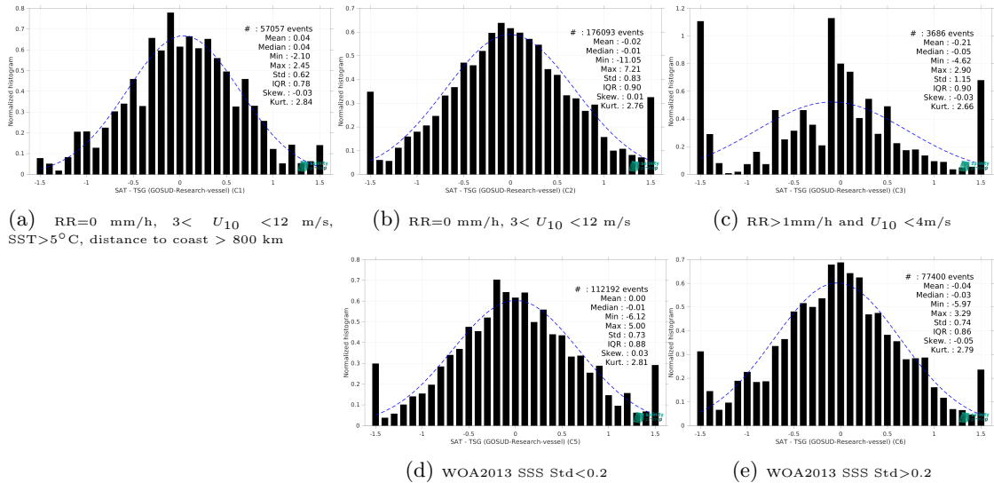
Figure 15: Normalized histogram of \Delta SSS (SMOS SSS L2 v700 (ESA) - TSG (GOSUD-Research-vessel)) for 5 different subdatasets corresponding to: RR=0 mm/h, 3 < U_{10} < 12 m/s, SST>5°C, distance to coast > 800 km (a), RR=0 mm/h, 3 < U_{10} < 12 m/s (b), RR>1mm/h and U_{10} < 4 m/s (c), WOA2013 SSS Std<0.2 (d), WOA2013 SSS Std>0.2 (e).
