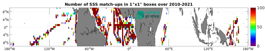
Figure 5: Number of SSS match-ups between TSG (GOSUD-Research-vessel) SSS and the SMOS SSS L2 v700 (ESA) SSS product for the Equatorial Ocean 10N-10S Pi-MEP region over 1^\circ \times 1^\circ boxes and for the full satellite product period.
