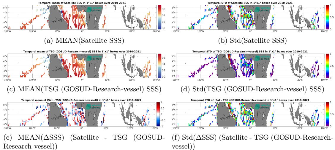
Figure 7: Temporal mean (left) and Std (right) of SSS from SMOS SSS L2 v700 (ESA) (top), TSG (GOSUD-Research-vessel) (middle), and of \Delta SSS (Satellite - TSG (GOSUD-Research-vessel)). Only match-up pairs are used to generate these maps.
