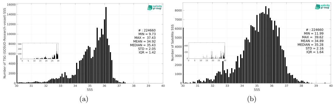
Figure 3: Histograms of SSS from TSG (GOSUD-Research-vessel) (a) and SMOS SSS L2 v700 (ESA) (b) considering all match-up pairs per bins of 0.1 over the Equatorial Ocean 10N-10S Pi-MEP region and for the full satellite product period.
